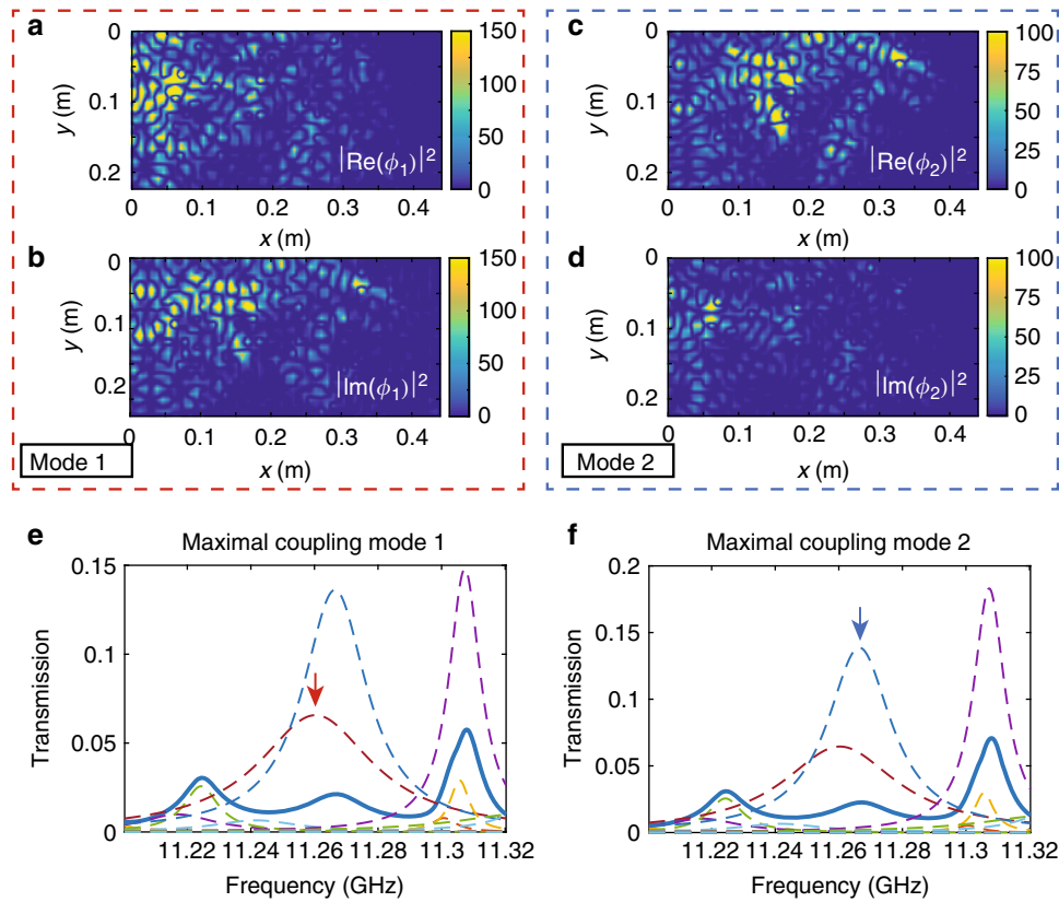
Fig. 5 Modal mixing. a–d The square of the real and imaginary parts, \text{Re}(\phi_n)^2 ( a , c ) and \text{Im}(\phi_n)^2 ( b , d ), of two strongly overlapping modes with resonance at f_1 = 11.260 GHz and f_2 = 11.266 GHz with linewidths \Gamma_1/(2\pi) = 21.7 MHz and \Gamma_2/(2\pi) = 12.3 MHz, respectively. e , f Transmission spectra (blue line) for maximal coupling to the first ( e ) and the second ( f ) mode. The dashed lines are the modal strengths. The small value of transmission in comparison to modal strengths in e , f is a result of strong destructive interference between the highly correlated speckle patterns of strongly overlapping modes
