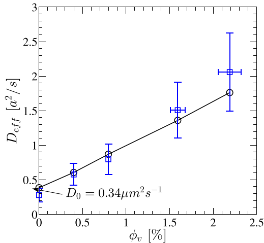
FIG. 6. Effective diffusion coefficient of tracers for the squirmer model with \beta = 0.5 . \ominus : simulations. \square : data from Leptos et al. (2009).
