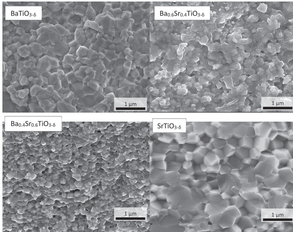
Fig. 2. FEG-SEM micrographs of \text{Ba}_{1-x}\text{Sr}_x\text{TiO}_{3-\delta} fractured dense ceramics.
