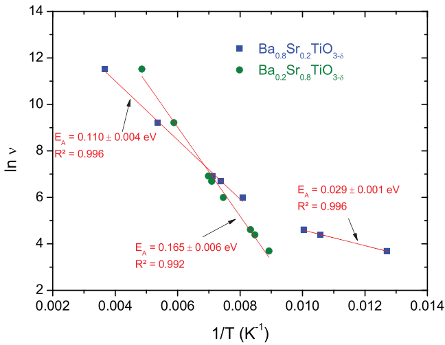
Fig. 7. Temperature dependence of relaxation frequency for \text{Ba}_{0.8}\text{Sr}_{0.2}\text{TiO}_{3-\delta} and \text{Ba}_{0.2}\text{Sr}_{0.8}\text{TiO}_{3-\delta} nanoceramics.
