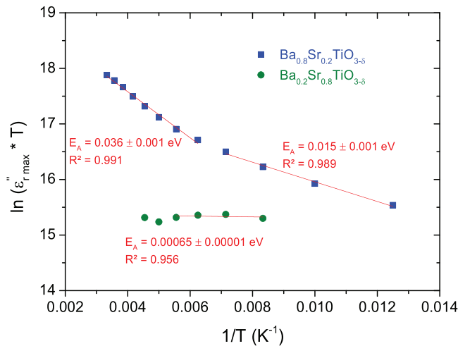
Fig. 10. Activation energy values extracted from the hopping polarons model for \text{Ba}_{0.8}\text{Sr}_{0.2}\text{TiO}_{3-\delta} and \text{Ba}_{0.2}\text{Sr}_{0.8}\text{TiO}_{3-\delta} nanoceramics.
