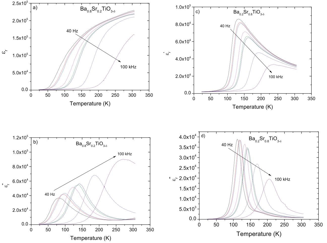
Fig. 6. Variation of the real parts (a) and (c) and the imaginary parts (b) and (d) of permittivity as a function of temperature and at different frequencies for \text{Ba}_{0.8}\text{Sr}_{0.2}\text{TiO}_{3-\delta} and \text{Ba}_{0.2}\text{Sr}_{0.8}\text{TiO}_{3-\delta} nanoceramics.
