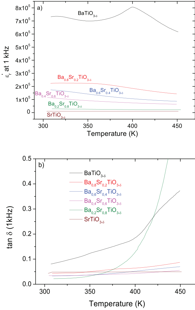
Fig. 5. Variation of the real part of the relative permittivity (a) and losses (b) as a function of temperature measured at 1 kHz for the \text{Ba}_{1-x}\text{Sr}_x\text{TiO}_{3-\delta} nanoceramics.
