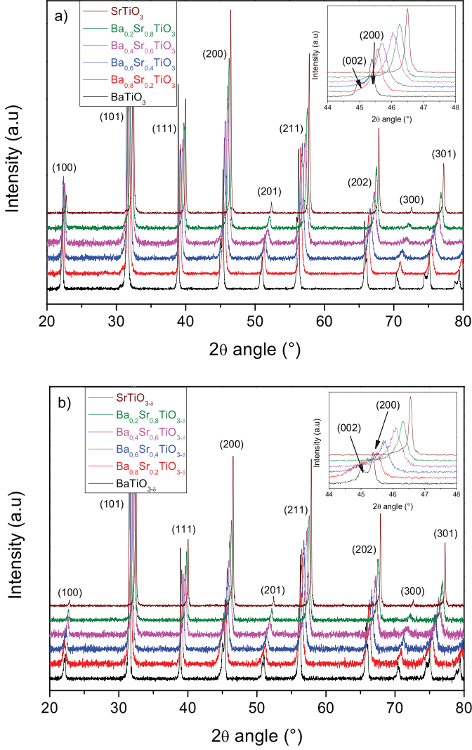
Fig. 3. XRD patterns of \text{Ba}_{1-x}\text{Sr}_x\text{TiO}_{3-\delta} (0 \leq x \leq 1 ) materials (a) powders and (b) ceramics; inset: 44–60° 2\theta angle enlargement.
