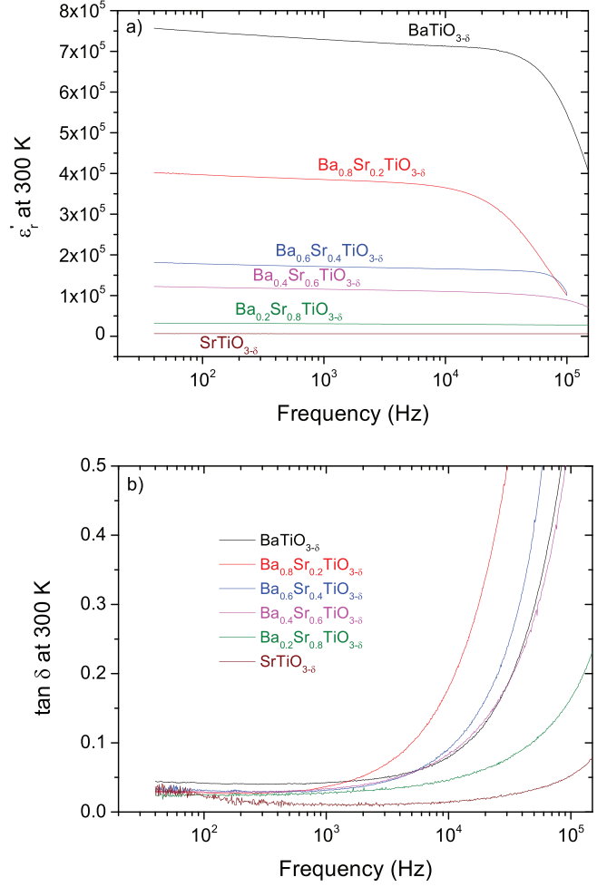
Fig. 4. Variation of the real part of relative permittivity (a) and losses (b) as a function of frequency for the \text{Ba}_{1-x}\text{Sr}_x\text{TiO}_{3-\delta} nanoceramics at 300 K.
