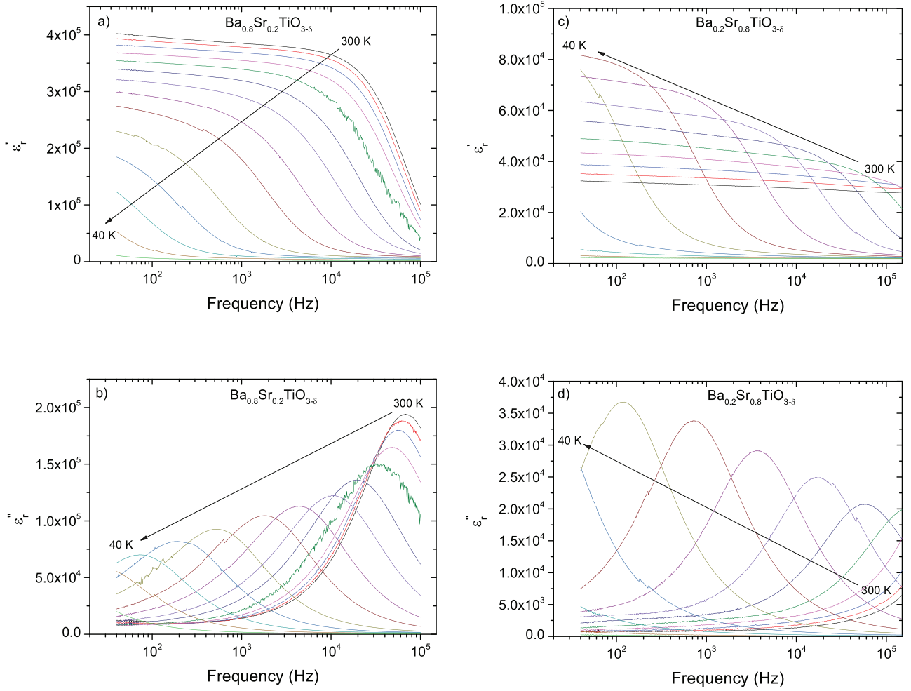
Fig. 8. Variation of the real part (a) and (c) and the imaginary part (b) and (d) of permittivity as a function of frequency and at different temperatures for \text{Ba}_{0.8}\text{Sr}_{0.2}\text{TiO}_{3-\delta} and \text{Ba}_{0.2}\text{Sr}_{0.8}\text{TiO}_{3-\delta} nanoceramics.
