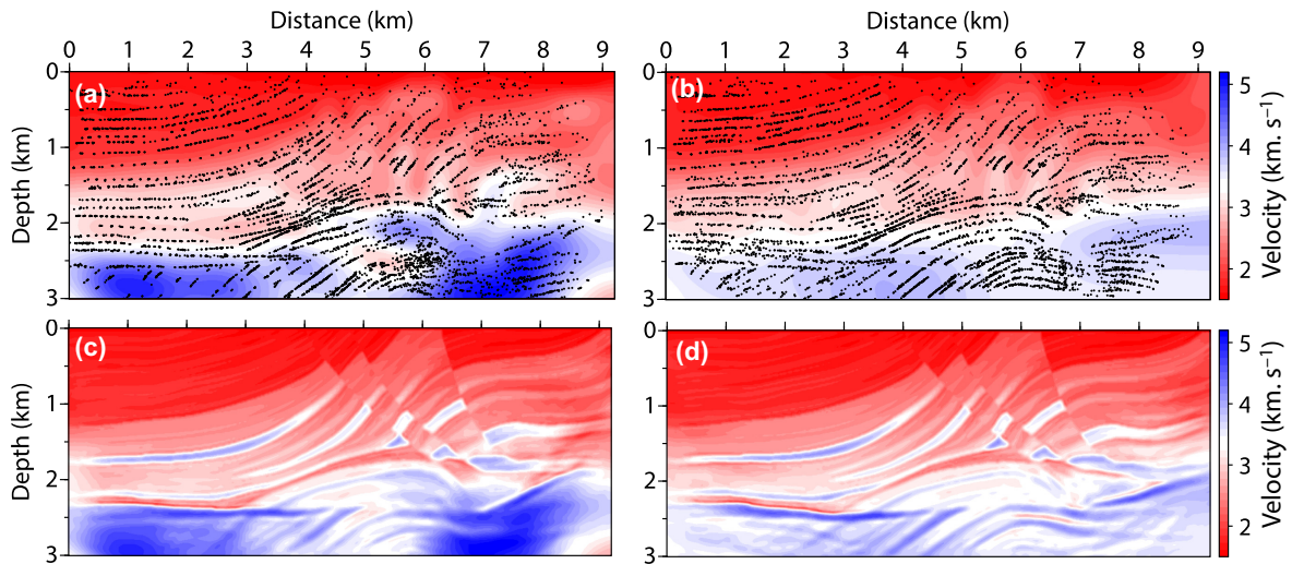
Figure 8. Marmousi example. (a) Velocity model inferred from 374 iterations of AST with superimposed scatterers (Tavakoli et al. 2017). (b) Velocity model inferred from 195 iterations of PAST with superimposed scatterers. In (a), scatterer coordinates were processed as optimization parameters in AST, while they were found by solving the focusing equations, eq. (12), in PAST. (c,d) Final FWI models obtained with initial models shown in (a) and (b).
