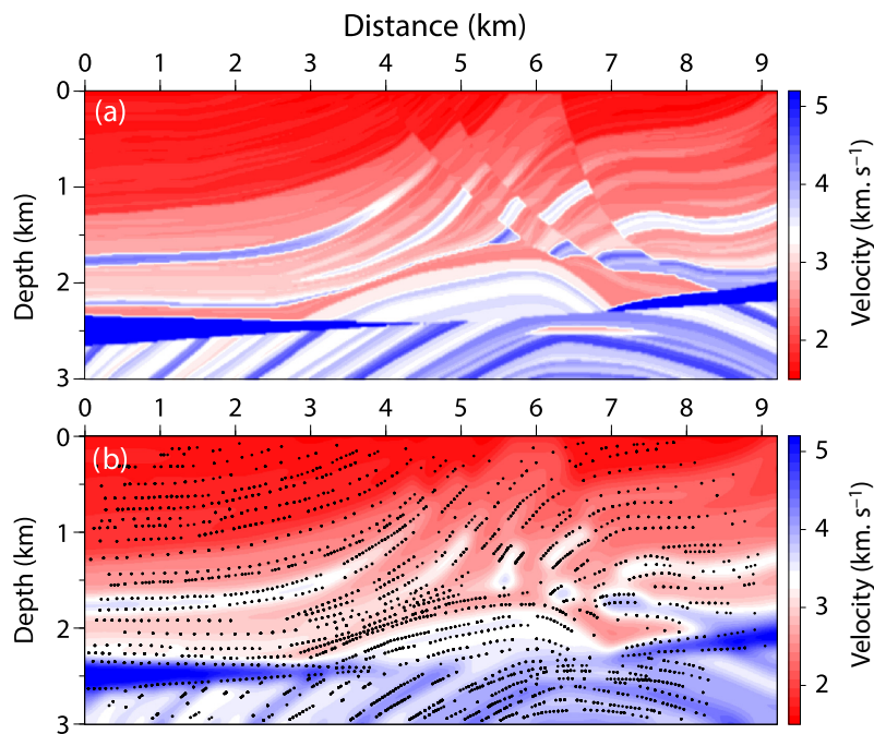
Figure 5. Marmousi example. (a) True blocky velocity model. (b) Picks of the Marmousi model reflectors. Picking was performed in the true velocity model shown in (a). Picks are superimposed on the smoothed velocity model that was used to generate the slope tomography measurements p_{S,n_{SF}}^* , T_{S,r,n_{S,r}}^* and p_{r,n_{SF}}^* by demigration.
