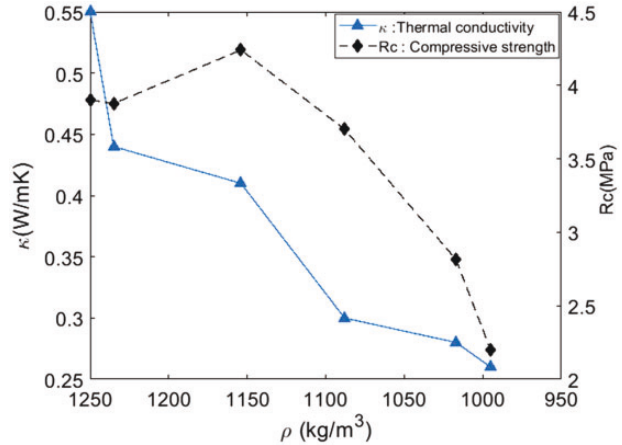
Figure 19. Compressive strength and thermal conductivity as a function of density.
