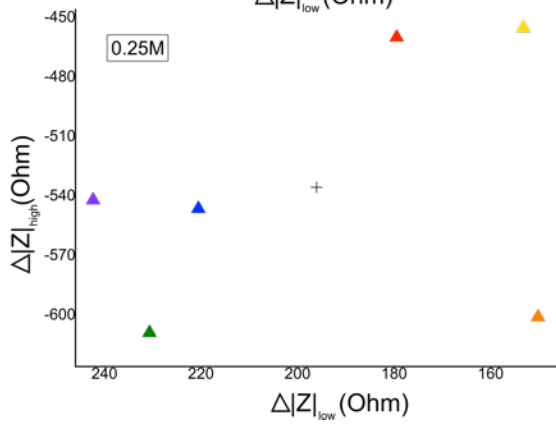
Fig. S9. Three dimensional plot of the low- and high-frequency impedance modulus variations with the ionic concentration under V_{DC} = -50 mV. Stacking of 1 M, 0.5 M, 0.25 M and 0.125 M planes, centered on their respective average point (cross point). Graphs of each concentration plane at 1 M; 0.5 M; 0.25 M and 0.125 M, function of \Delta|Z|_{low} and \Delta|Z|_{high} .
