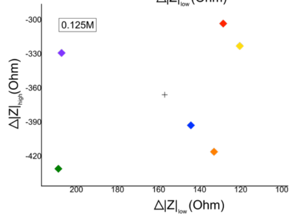
Fig. S9. Three dimensional plot of the low- and high-frequency impedance modulus variations with the ionic concentration under V_{DC} = -50 mV. Stacking of 1 M, 0.5 M, 0.25 M and 0.125 M planes, centered on their respective average point (cross point). Graphs of each concentration plane at 1 M; 0.5 M; 0.25 M and 0.125 M, function of \Delta|Z|_{low} and \Delta|Z|_{high} .
