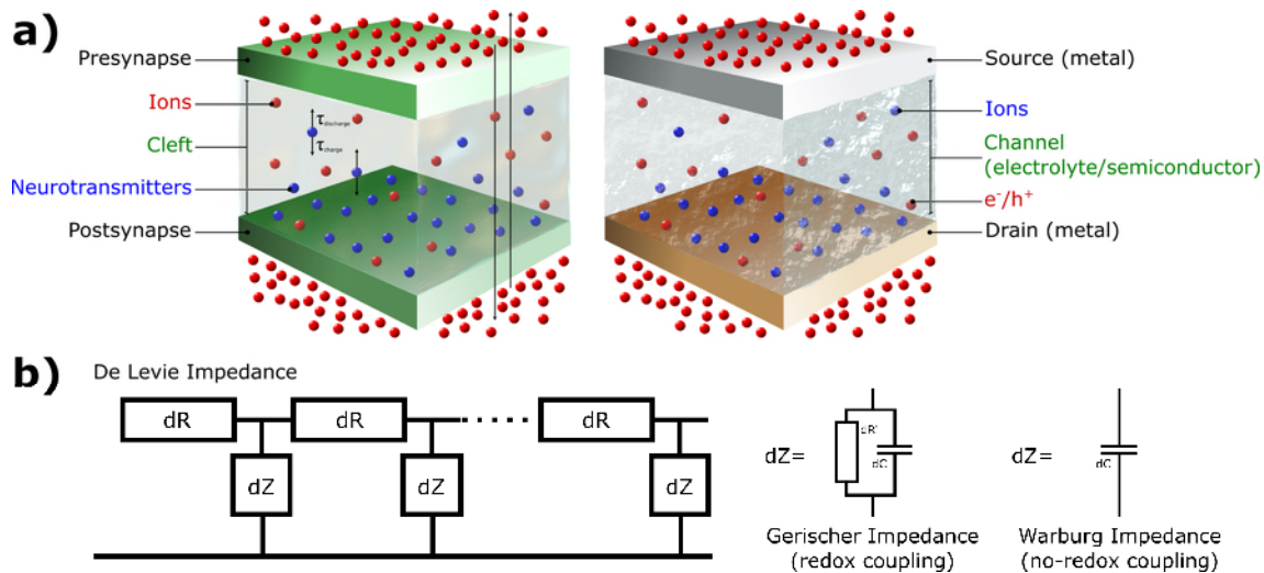
Figure 2: (a) Analogy between a biological synapse and organic-electrochemical synapse. (b) De Levie infinite transmission line impedance model for porous electrode with redox (Gerischer Impedance) or without redox (Warburg Impedance) reaction.
