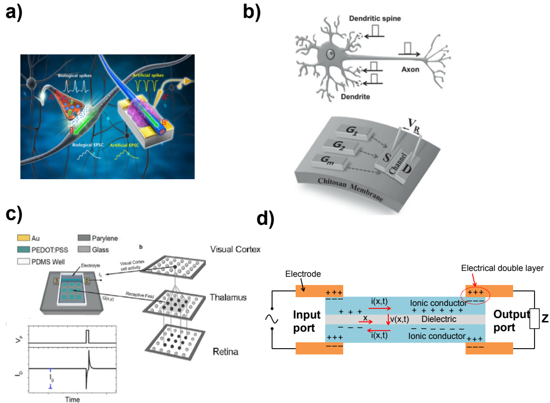
Figure 3: (a) Organic dendrites and synapses realized by inkjet printing of organic core-sheath nanowire (from [83]). (b) Emulation of dendritic propagation of signals with IZO transistor and chitosan ionic membrane (adapted from [85]). (c) Orientation selectivity with dendritic-like organic electrochemical transistors (adapted from [84]). (d) Concept of ionic cable (adapted from [86]).
