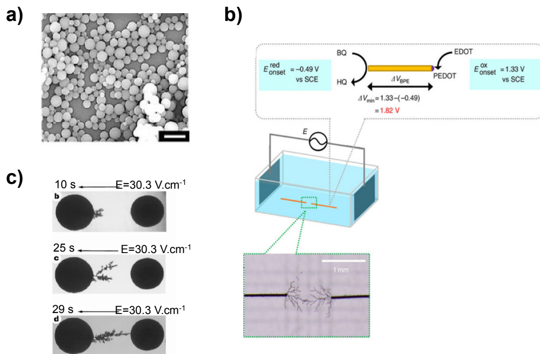
Figure 5: (a) Assembling of conducting polymer microspheres (adapted from [92]), scale bar is 5μm. (b) Dendritic PEDOT:PSS interconnection (adapted from [97]). (c) Electrical interconnection of microspheres (adapted from [99]).
