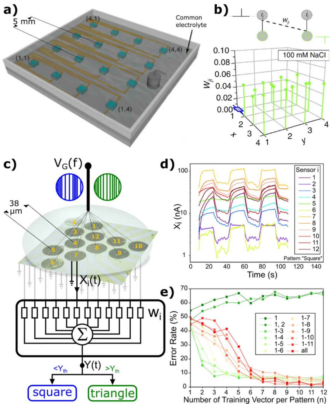
Figure 4: (a-b) Global gating through the electrolyte of organic electrochemical transistors showing both local and global tenability of the devices (adapted from [87]). (c-d) Concept of spatial reservoir implemented with electropolymerized OECTs for pattern classification (adapted from [88])
