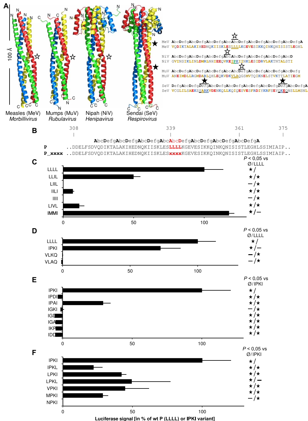
Fig. 3. Conservation of deformations in the coiled coil of P MD within paramyxoviruses and functional impact of substitutions within the stammer of MeV P. (A) Ribbon representation of the crystal structures of the P MDs from MeV (PDB code 3ZDO), MuV (PDB code 4EIJ) (note its particular antiparallel orientation), NiV (PDB code 4GJW), and SeV (PDB code 1EZJ), four Paramyxoviridae members representative of four genera. Kinks induced by insertion of stammers (i.e., insertion of three extra amino acids) or stutters (i.e., insertion of four extra amino acids) that disrupt the heptad regularity of the coiled coil are indicated by empty and full stars, respectively. (B) Amino acid sequences and register of the P MDs from MeV, NiV, MuV, and SeV. For the amino acids out of register, a register was manually assigned according to the expected register resulting from the insertion of either a stammer or a stutter (letters in italics). Stammers and stutters are underlined, and the residues of the kinks are highlighted by empty or full stars for stammer- or stutter-induced kinks, respectively. (C) Sequences of kink variants with the expected heptad register. (D to F) Activity in a minigenome assay of P stammer variants bearing mutations with hydrophobic residues (C), replacement with other paramyxovirus stammers (D), and mutations of exposed (E) or buried residues (F) of IPKI. BSR-T7 cells were transfected with the mixture of expression vectors encoding the minigenome, N, L, and P variants. The firefly luciferase activity was measured 2 days after transfection. Data are means ± SD of at least three independent experiments, with each point done in triplicate. Statistically significant differences (Student's t test) at P < 0.05 and below with respect to the negative "∅" and positive LLLL or IPKI controls are quoted by stars.
