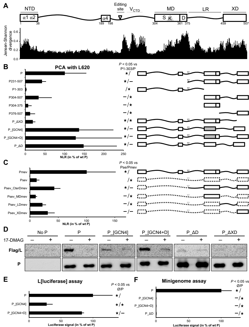
Fig. 1. MeV P organization in conserved modules responsible for binding, stabilizing and supporting L. (A) Top: NTD with \alpha 1\alpha 2 and \alpha 4 helix-prone regions involved in N^0P complex formation. LR, linker region. MD can be subdivided into two regions: a stable S module (amino acids 304 to 360) and a dynamic D module (amino acids 361 to 375), with former including a kink (K). P mRNA editing site and the region of P overlapping with V protein C-terminal domain ( V_{CTD} ) are also shown. Bottom: Conservation score for each amino acid of MeV P calculated on the basis of Jensen-Shannon divergence (32) with an alignment of amino acid sequence of P from at least one member of each genus of the Paramyxoviridae family recorded in National Centre for Biotechnology Information (NCBI) databank with the following accession numbers: HQ385703, KF687315, KP171417, KT749883, MF795094, LC000638, EU439428, NC_028362, MG573141, MG516455, KX940962, KY370098, NC_007454, MG573140, KJ641657, KC154054, NC_002199, MF943130, NC_005339, NC_017937, KY971532, JN234009, EU267273, Z47758, MF627832, JN255804, FN869553, NC_025351, NC_025256, NC_025347, NC_025361, KP762799, KX258200, MF033136, JX901129, NC_025349, EU338414, NC_034968, NC_025407, GQ338311, KX119151, NC_025363, NC_025390, MF594598, KY452444, KY452443, KY452442, JN571485, NC_025373, KX953297, NC_003443, NC_006428, AJ749976, NC_021928, KX064232, KT213728, NC_009489, NC_004074, JX112711, NC_025403, NC_025348, NC_025350, NC_025343, NC_025404, NC_025410, KJ641654, JF795583, NC_025360, NC_005084, and MH411104. (B and C) Truncated and chimeric P binding to L620 protein as measured by Gaussia luciferase–derived PCA. P constructs are fusion proteins, with the first domain of the Gaussia luciferase (glu1) fused to their N terminus except for the 1–303 fragment, where glu1 was grafted at the C terminus. L620 was grafted with the second domain of the luciferase (glu2) at its N terminus. 293T cells were transfected to coexpress glu2-L620 with a glu1-P variant. Gaussia luciferase activity was measured 24 hours after transfection. Normalized luminescence ratio (NLR) was calculated for each condition. Results are shown in percentage of wt P NLR. P_[GCN4] and P_[GCN4+D] have the S region of their MD substituted with a tetramerization domain derived from the yeast GCN4 transcription factor. (D) Ability of P variants to assist L folding by the HSP90 chaperon as monitored by SDS–polyacrylamide gel electrophoresis and Western blot in the absence (–) and presence (+) of the HSP90 inhibitor 17-DMAG. Note the very poor expression level of Flag/L in the absence of P (“no P” panel). (E) P variant ability to assist L folding as measured using an L[luciferase] folding assay (30). The principle is that the folding, and consequently the enzymatic activity, of the luciferase embedded in the middle of the L protein relies on the appropriate folding of the upstream L region. Hence, the level of luciferase activity reflects both the amount of L and the quality of its folding in the presence of each P variant. (F) P variant activity in a luciferase-based minigenome assay. BSR-T7 cells were transfected with the mixture of expression vectors encoding the minigenome, N, L, and P variants. The firefly luciferase activity was measured 2 days after transfection. Data in (A), (B), (D), and (E) are means \pm SD of at least three independent experiments, with each point done in triplicate. Statistically significant differences (Student’s t test) at P < 0.05 and below, with respect to the negative “Ø” (unless otherwise indicated) and positive “wt” P (unless otherwise indicated) control, are quoted by stars. Although not below the 0.05 threshold, P values for Psev_LDmev versus Psev, Psev_XDmev versus Psev, and Psev_XDmev versus Pmev are 0.096, 0.064, and 0.07, respectively.
