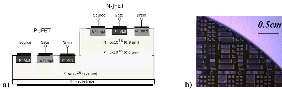
Fig. 1. Cross-sectional structure of the integrated P and N lateral JFET (a), optical micrographs recorded after the technological fabrication process (b)
