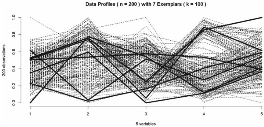
Fig. 1. Profiles of 200 simulated data with 5 variables (dashed lines) election of 7 exemplars with a parameter value k = 100 (bold lines)
