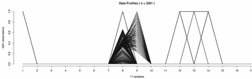
Fig. 3. Profiles of 3 201 data with 17 variables from roadway experimentation.
