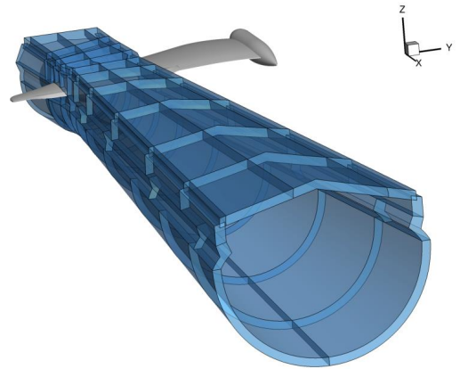
Figure 7: Illustration of the CFD/CAA chaining volumes.
