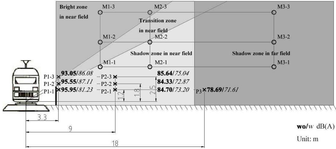
Fig. 2 Configurations of the in-situ experiments with the straight barrier on the ground line (frequency range: 20-20 kHz)
