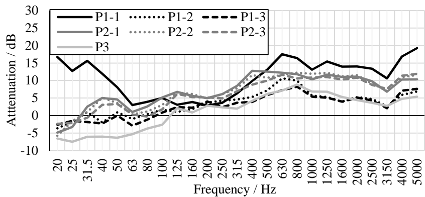
Fig. 4 Attenuations in the one-third-octave band at all receiver positions (20-5000Hz)
