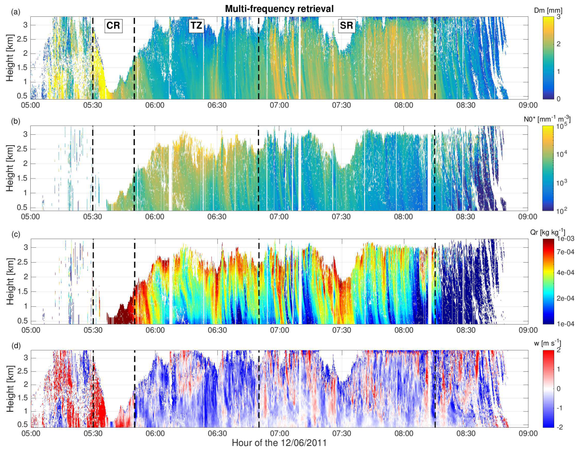
FIG. 8. Time-height evolution of some of the retrieved parameters: (a) mean volume diameter D_m , (b) concentration parameter NO^* , (c) rain mixing ratio q_r and (d) vertical wind w . The vertical lines indicate the three different periods of the squall line determined from Figure 5.
