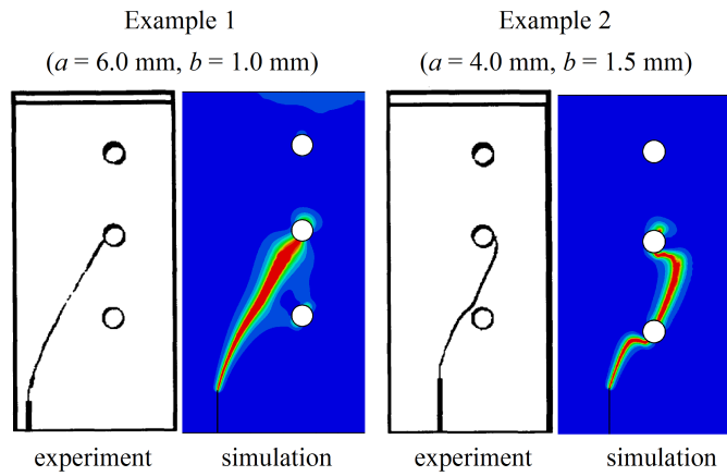
Figure 16: Fracture pattern for the two cases compared with experimental results of Bittencourts et al. [33].
