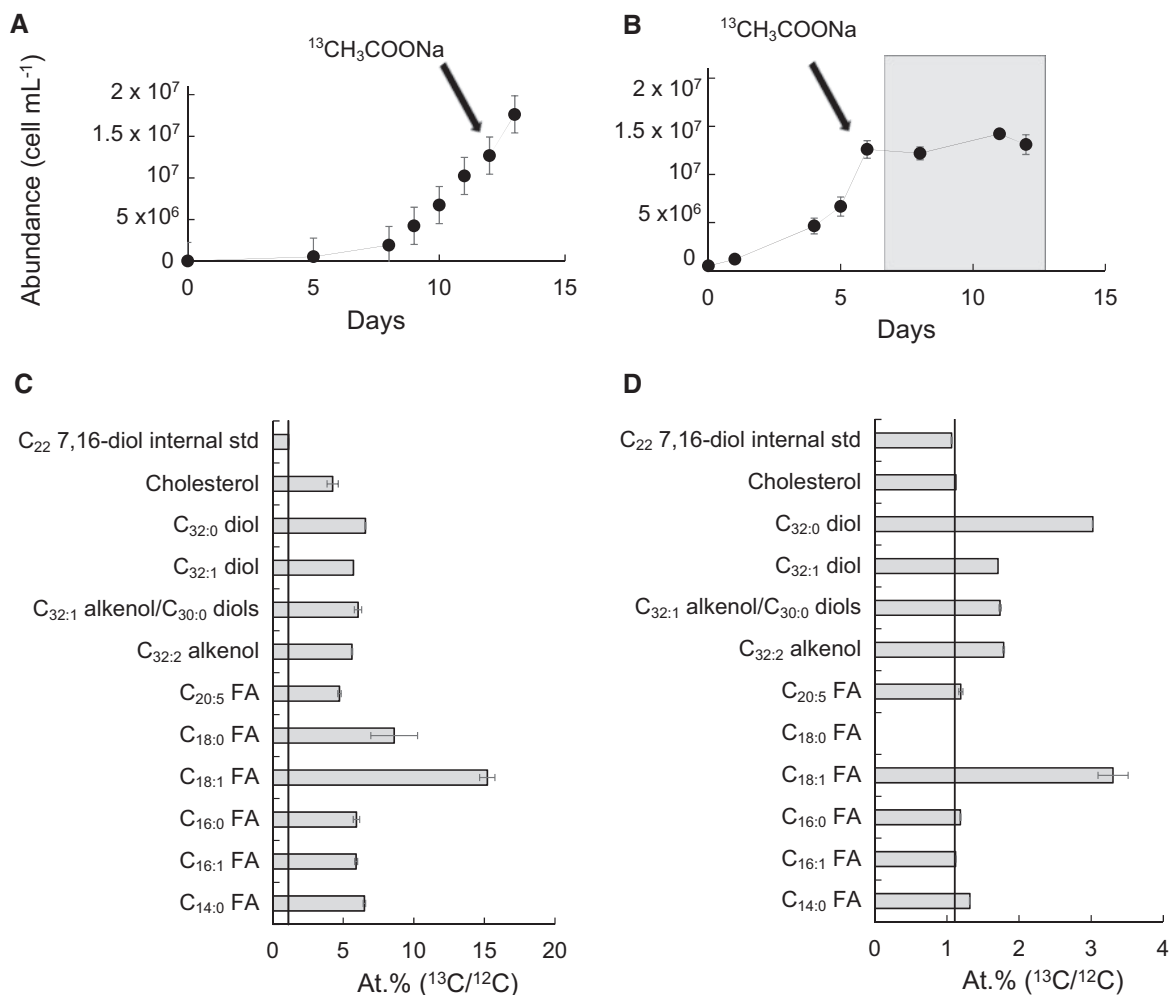
Fig. 2 Incorporation of ^{13}\text{C} -labelled sodium acetate in the biomass of N. oceanica CCMP1779 under dark/light (A, C), and dark (B, D) conditions. Growth curves (A, B) depicting the cell abundance of the culture during the experiment. The grey area denotes the time interval of dark incubation whereas arrows indicate the supply of ^{13}\text{C} -labelled sodium acetate. Atomic ^{13}\text{C} percentage (of ^{13}\text{C}+^{12}\text{C} ) (C, D) measured by GC-IR-MS for selected lipids at the end of the experiment. Error bars represent the standard deviation calculated from three replicate measurements on the lipid extract (note that some error bars are too small to be visible in the graph). The straight line indicates the natural atomic ^{13}\text{C} percentage.
