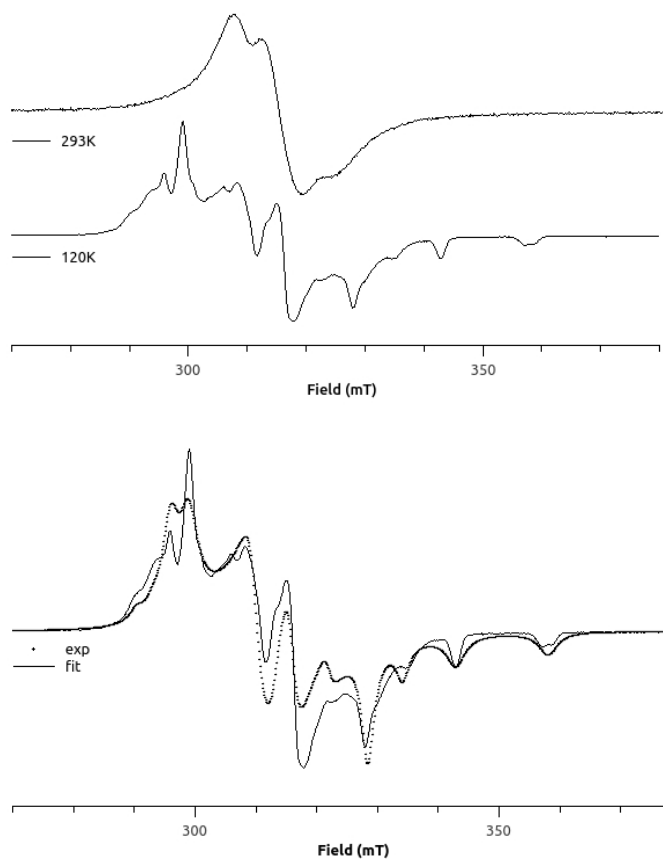
Figure 4. Experimental (MeCN/toluene, 293 K, and \text{CH}_2\text{Cl}_2 /toluene, 120 K, top ), and simulated (120 K, bottom ) X-band EPR spectra of 4 .
