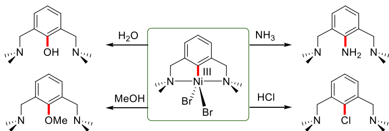
Scheme 2. Previous work on C-heteroatom coupling promoted by a \text{Ni}^{\text{III}} precursor.
