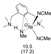
Scheme 15. (a) Lowest free energy (and enthalpy) landscape for reaction of 3 with \text{CH}_3\text{NH}_2 . (b) A representative example of the higher energy transition states examined (kcal/mol).
