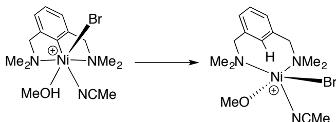
Scheme 11. Possible protonation of the aryl moiety by CH 3 OH
