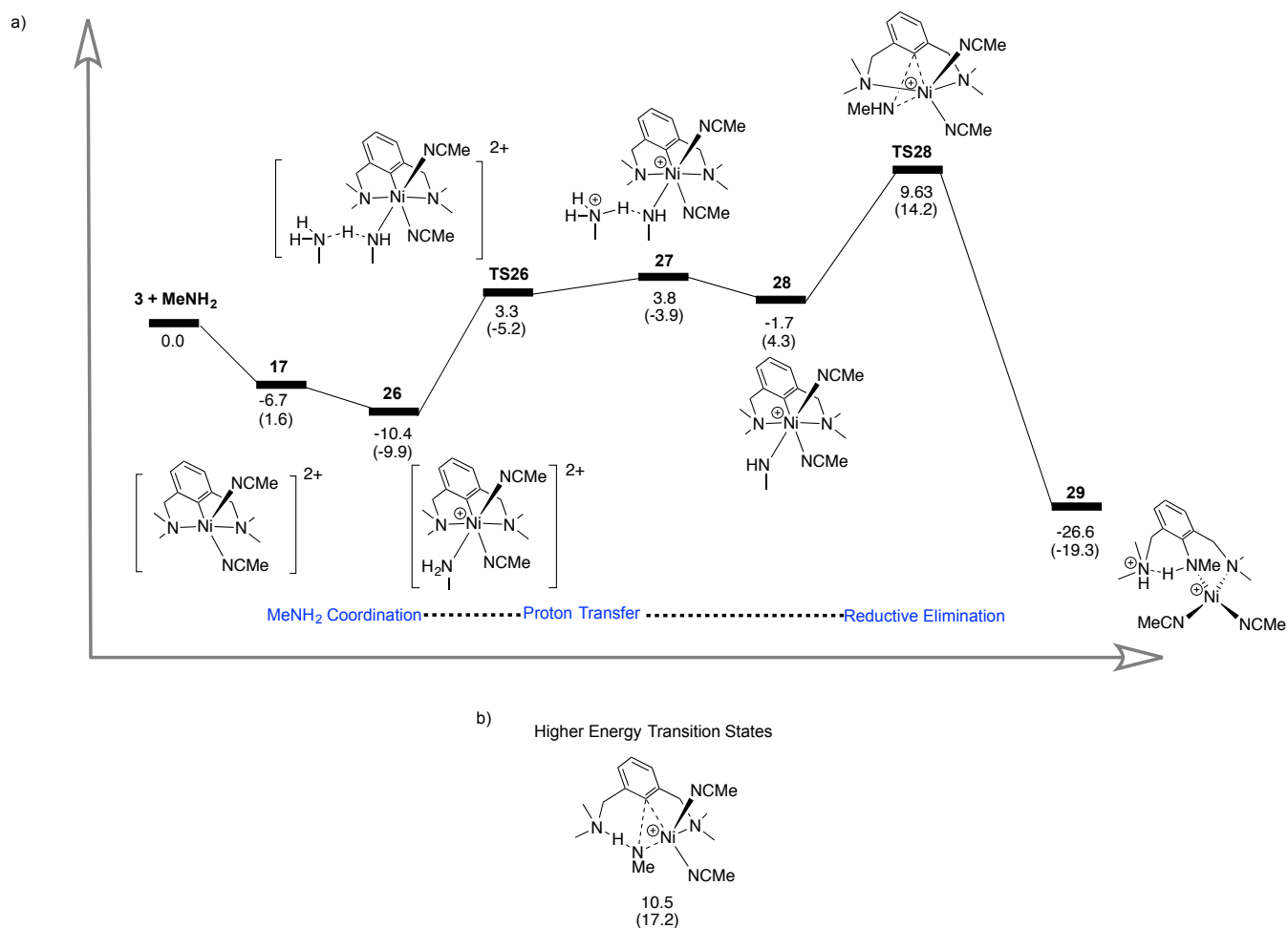
Scheme 15. (a) Lowest free energy (and enthalpy) landscape for reaction of 3 with CH 3 NH 2 . (b) A representative example of the higher energy transitions states examined (kcal/mol).
