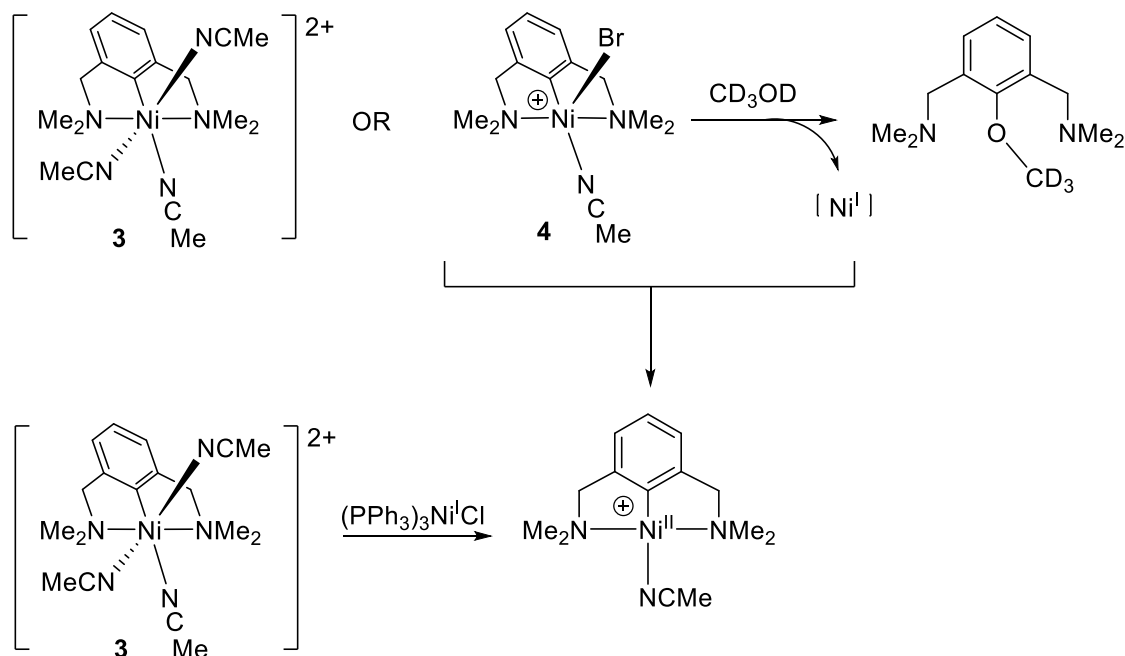
Scheme 6. Reactivities of 3 and 4 in support of proposed functionalization mechanism.
