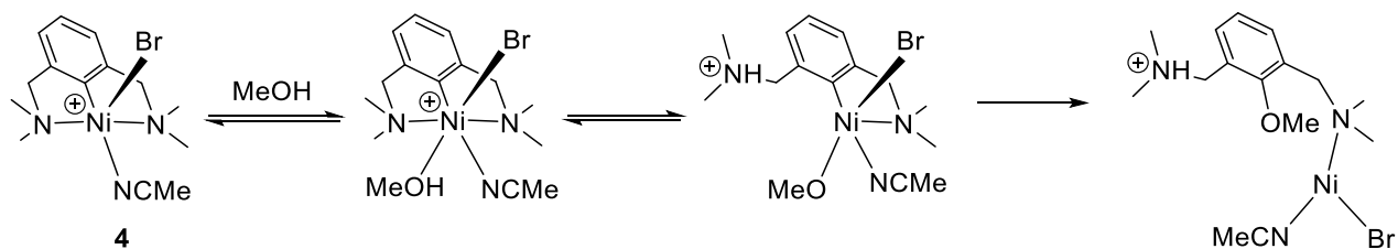
Scheme 8. Simplified mechanistic proposal for C-O coupling for reaction between 4 and \text{CH}_3\text{OH} .
