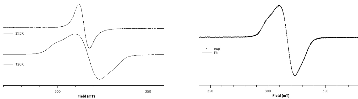
Figure 3. Experimental (MeCN, 293 and 120 K, left ), and simulated (120 K, right ) X-band EPR spectra of 3 .
