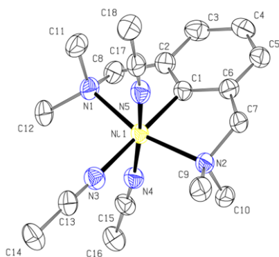
Figure 1. X-ray structure of 3 . Thermal ellipsoids are shown at the 50% level. The \text{SbF}_6 counter anions and all H atoms are omitted for clarity. Selected bond distances (Å) and angles (°): Ni1-N1 = 2.122(4); Ni1-N2 = 2.099(4); Ni1-N3 = 2.003(5); Ni1-N4 = 2.082(5); Ni1-N5 = 2.086(5); Ni1-C1 = 1.905(5); N1-Ni1-N2 = 161.34(17); C1-Ni1-N3 = 179.2(2); Ni1-N3-C13 = 177.5(5); Ni1-N4-C15 = 170.6(5); Ni1-N5-C17 = 169.4(5).
