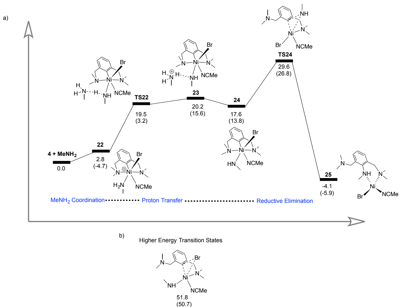
Scheme 14. Lowest free energy (and enthalpy) landscape for the reaction of 4 with \text{CH}_3\text{NH}_2 . (b) A representative example of the higher energy transitions states examined (kcal/mol).
