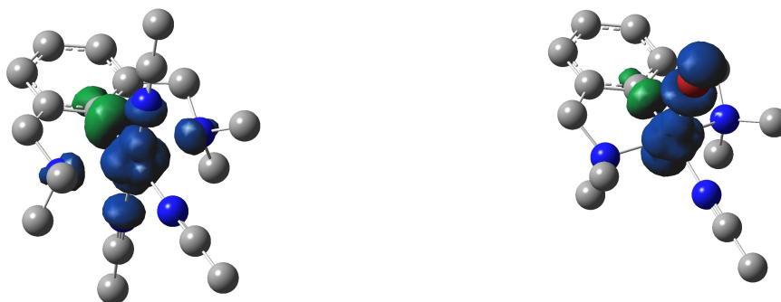
Figure 5. Alpha spin density plots for complexes 3 ( left ) and 4 ( right ). Plots generated with an isovalue of 0.004 \text{ e}/\text{\AA}^3 .
