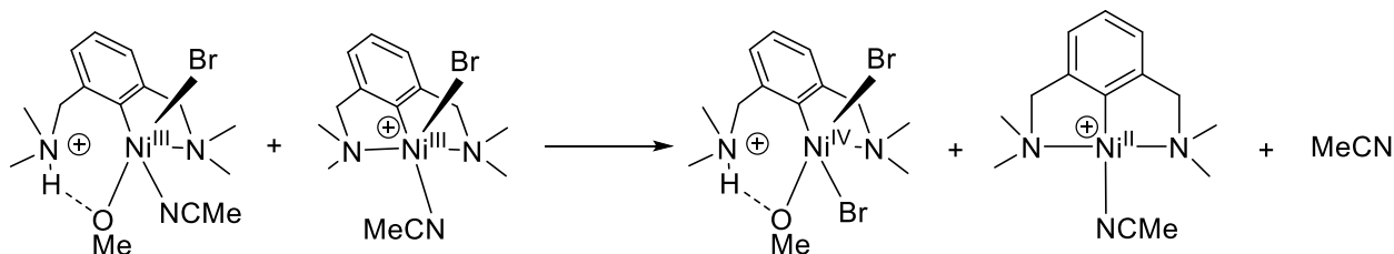
Scheme 12. Possible disproportionation reaction between two Ni III complexes
