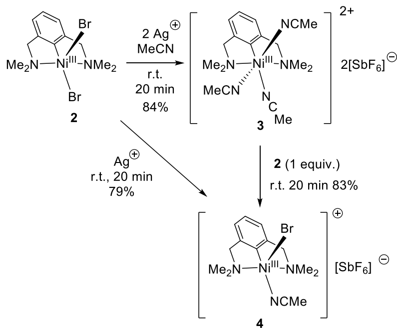
Scheme 4. Syntheses of [(NCN)Ni III (MeCN) 3 ] 2+ 2[SbF 6 ] - ( 3 ) and [(NCN)Ni III (Br)(MeCN)] + [SbF 6 ] - ( 4 ).
