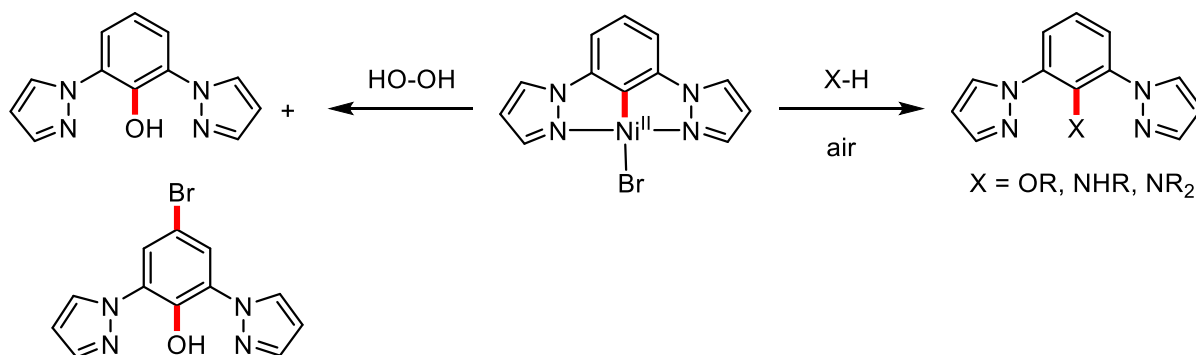
Scheme 1. Previous work on C-heteroatom coupling promoted by a \text{Ni}^{\text{II}} precursor.
