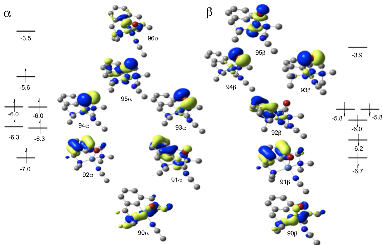
Figure 7. UM06L \alpha -spin and \beta -spin molecular orbitals for monocationic complex 4 . Orbital energies reported in eV.
