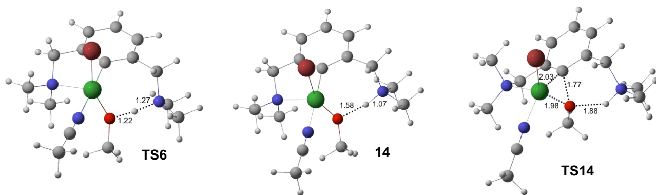
Figure 9. 3D representations of proton transfer and reductive elimination transition states for the reaction of 4 with CH 3 OH. Bond and partial bond lengths reported in Å.
