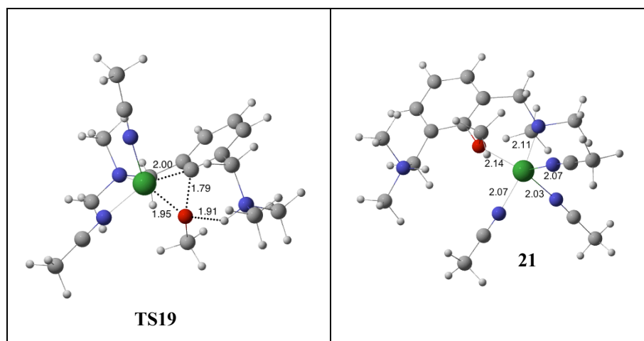
Scheme 13. Lowest free energy landscape for (and enthalpies) for reaction of 3 with CH 3 OH.
