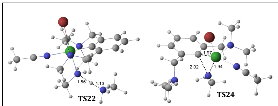
Figure 11. 3D representations of proton transfer and reductive elimination transition states for the reaction of 4 with \text{CH}_3\text{NH}_2 . Bond and partial bond lengths reported in Å.
