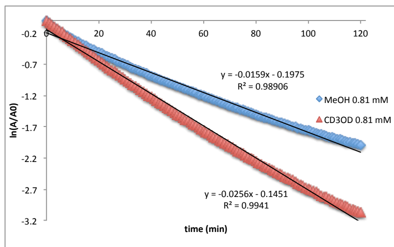
Figure 6. UV-visible spectroscopy time course profile for the reaction of a 0.81 mM solution of 4 with CH 3 OH/CD 3 OD.
