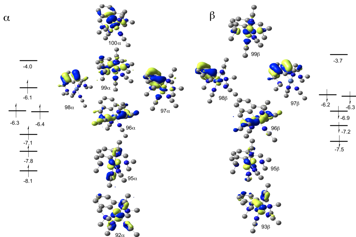
Figure 8. UM06L \alpha -spin and \beta -spin molecular orbitals for dicationic complex 3 . Orbital energies reported in eV.
