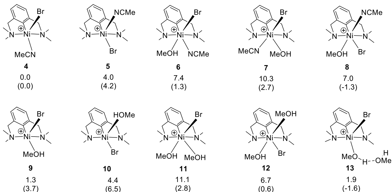
Scheme 9. Gibbs free energy (and enthalpy) for CH 3 OH coordination and substitution with complex 4 . (kcal/mol)
