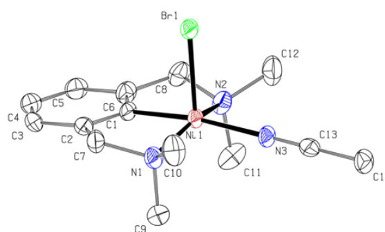
Figure 2. X-ray structure of 4 . Thermal ellipsoids are shown at the 50% level. The \text{SbF}_6 counter anion and all H atoms are omitted for clarity. Selected bond distances (Å) and angles (°): Ni1-N1 = 2.013(4); Ni1-N2 = 2.011(4); Ni1-C1 = 1.873(4); Ni1-N3 = 1.978(4); Ni1-Br1 = 2.4014(8); N1-Ni1-N2 = 156.06(17); C1-Ni1-N3 = 171.56(16); C1-Ni1-Br1 = 90.31(12).
