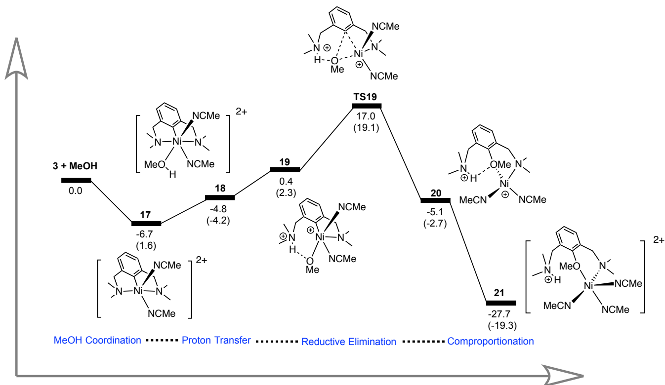
Scheme 13. Lowest free energy landscape for (and enthalpies) for reaction of 3 with CH 3 OH.
