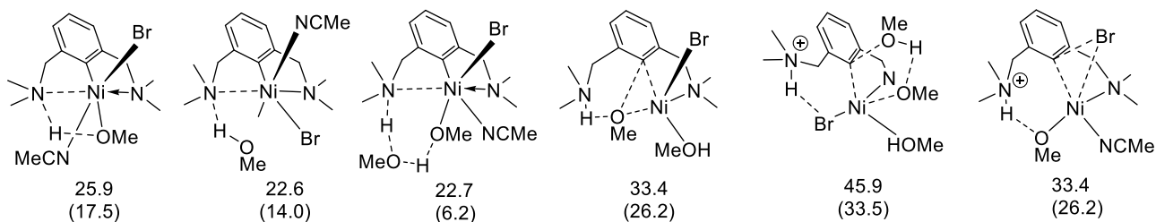
Scheme 10. a) Lowest free energy (and enthalpy) landscape for reaction of 4 with CH 3 OH. (b) Representative examples of higher energy transition states examined (kcal/mol).
