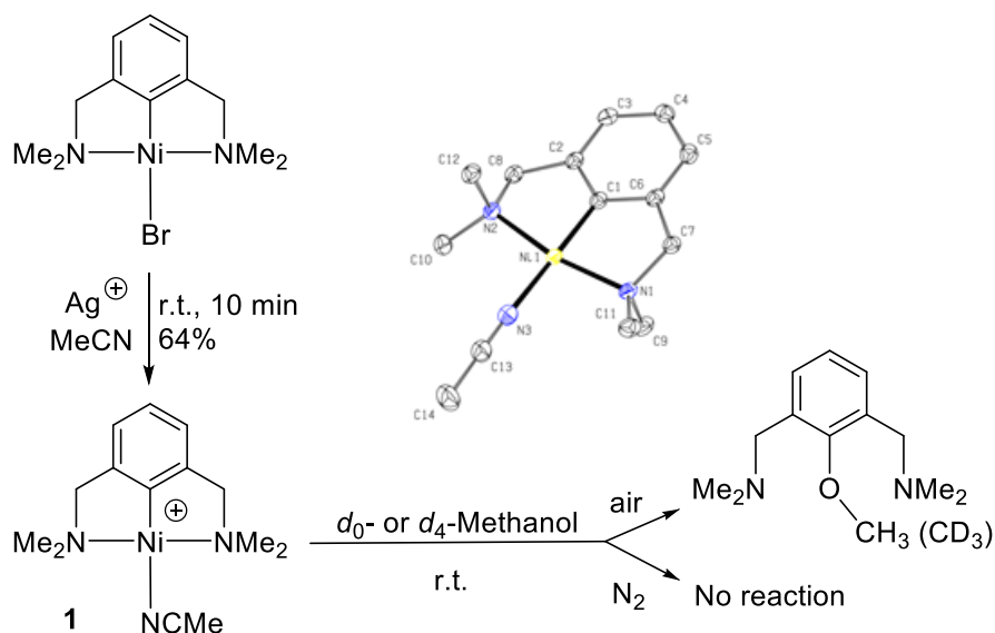
Scheme 3. Synthesis of [(\text{NCN})\text{Ni}^{\text{II}}(\text{MeCN})]^+ ( 1 ) and its reaction with methanol.
