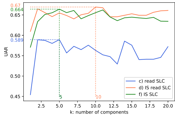
Fig. 5. Performances of the ASIMPLS systems with the best b' depending on the number of components k on train vs dev
