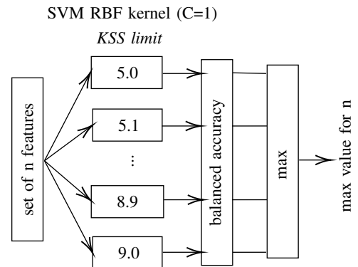
Fig. 3. Flowchart of the gridsearch to compute the best performance with n features. The SVM are trained with the train dataset and tested with the development dataset.
