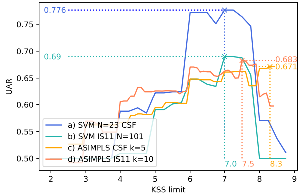
Fig. 7. Sensitivity of the system to the limit of the KSS on the read tasks of the SLC.
