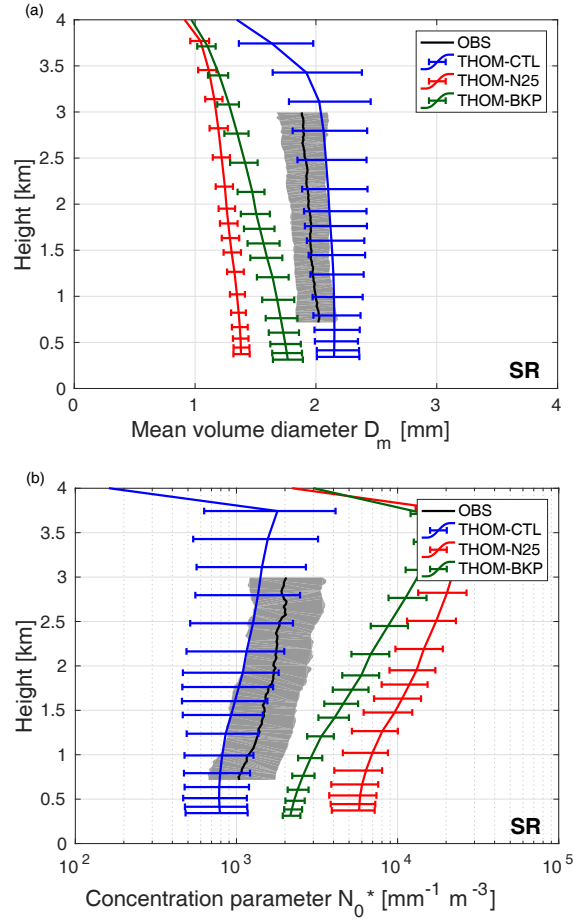
FIG. 4. As in Figure 3, but for THOM-CTL, THOM-N25 and THOM-BKP simulations.
