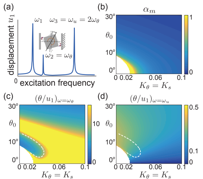
Figure 2. Eigenfrequencies and eigenvectors of the considered metasurface. In the linear dissipative regime, three resonance frequencies \omega_i ( i = 1, 2, 3 ) are presented (a), related to either a translation-dominated movement, denoted \omega_u , or a rotation-dominated movement denoted \omega_\theta , or a combination of both. When the resonance frequency condition \omega_u = 2\omega_\theta is satisfied, the mass ratio \alpha_m is determined for different values of initial angles of rotation \theta_0 and stiffnesses K_s and K_\theta (b). The ratio of \theta to U_1 is examined as a function of \theta_0 and K_s = K_\theta as well, at resonance frequencies \omega_\theta and \omega_u in (c) and (d), respectively. The optimal value range of stiffness and initial angle of rotation is indicated by the white dotted line in both (c) and (d).
