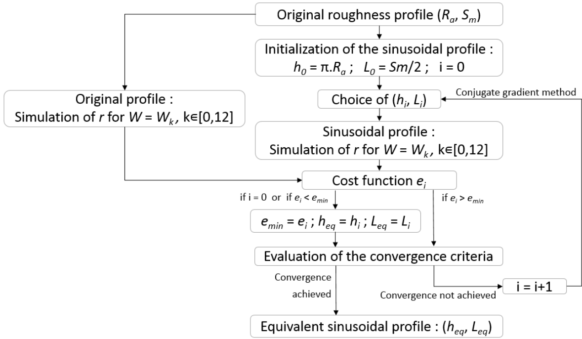
Fig. 2: Schematical description of the optimization method aiming at determining the equivalent sinusoidal roughness profile (with parameters h_{eq} , L_{eq} ) corresponding to each original roughness profile (with parameters R_a , S_m ).
