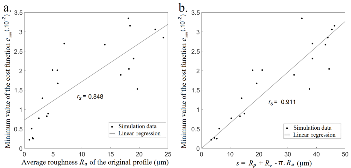
Fig.11: Variation of the minimum value of the cost function e_{min} as a function of (a) the average roughness of the implant R_a and (b) s = R_p + R_v - \pi \cdot R_a . The solid lines correspond to a linear regression analysis.
