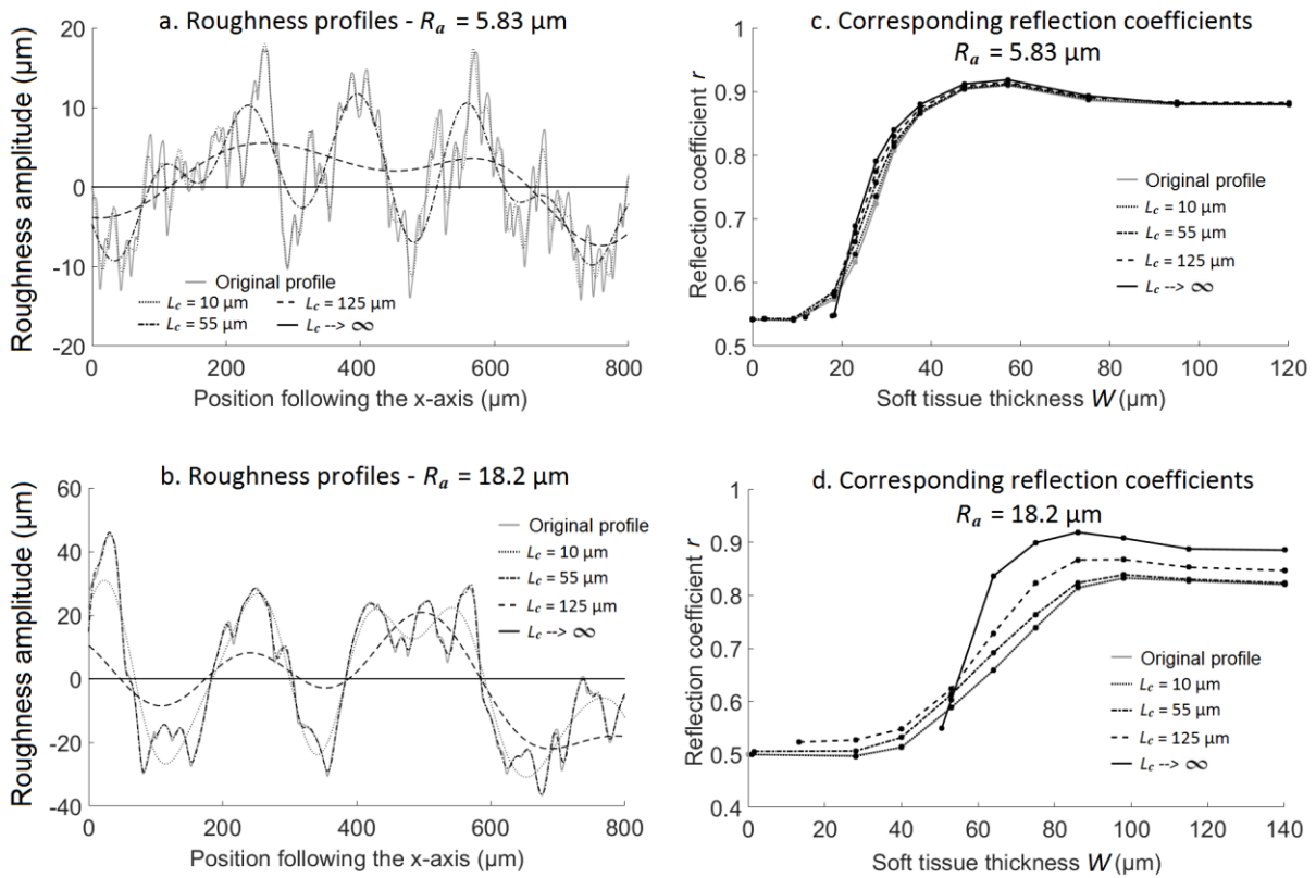
Fig. 5: Roughness profiles of an implant surface with (a) R_a = 5.83 \mu\text{m} and (b) R_a = 18.2 \mu\text{m} together with the corresponding profiles filtered with different values of the cut-off
