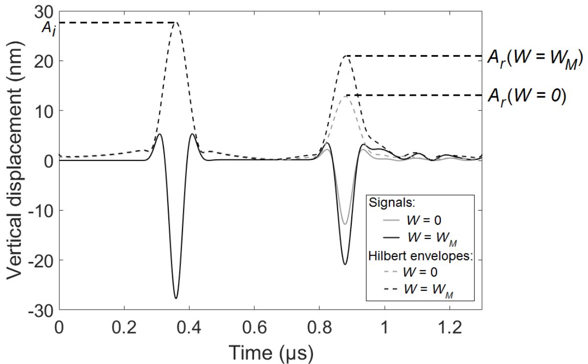
Fig. 3. Radiofrequency signals (solid lines) with their envelopes (dashed lines) corresponding to the ultrasonic waves recorded at H_{Ti}/2 and averaged over x for an implant surface with R_a = 24.2 \mu m in the cases of fully-bonded ( W = 0 ) and fully debonded ( W = W_M ) interfaces.
