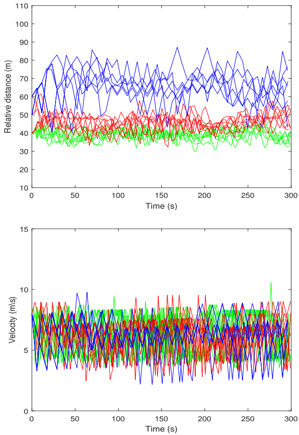
Fig. 8: Simulation results of a platoon of 20 vehicles on a circular road with different sampling periods: inter-vehicle distance (top), velocities (bottom)(green: vehicles with different sampling periods in [1.9, 2.02] , red: vehicles with different sampling periods in [3.4, 3.52] , blue: vehicles with different sampling periods in [5.7, 5.8] ).
