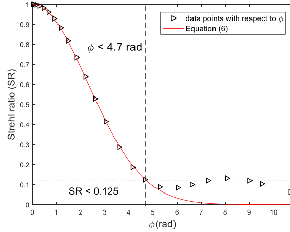
Fig. 3. SR versus optical phase difference ( \phi ). The red curve represents Eq. (6).
