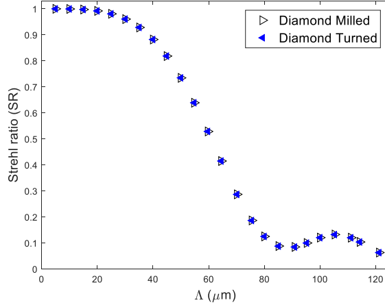
Fig. 2. The impact of diamond machined MSF errors on the SR with respect to groove spacing for the specific case study. Simulation results indicate similar SR values for diamond-milled and diamond-turned optics (RMSE=0.000172).
