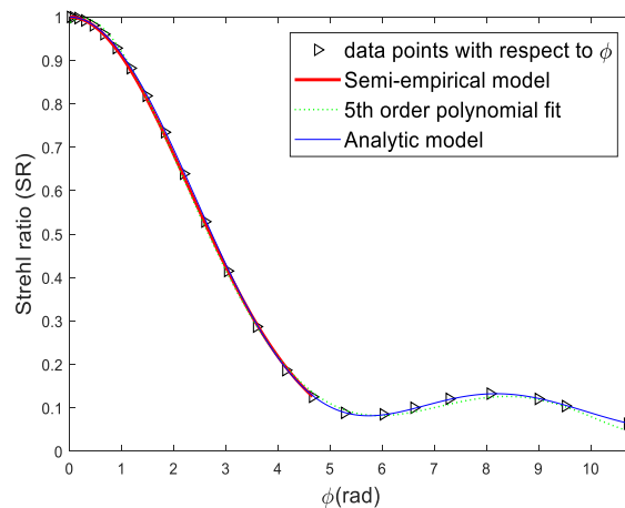
Fig. 4. Comparison of the semi-empirical and analytic SR expressions, given by Eq. (6) and (1), respectively. For \phi < 4.7 rad, the two models differ by a RMSE of 0.0058.
