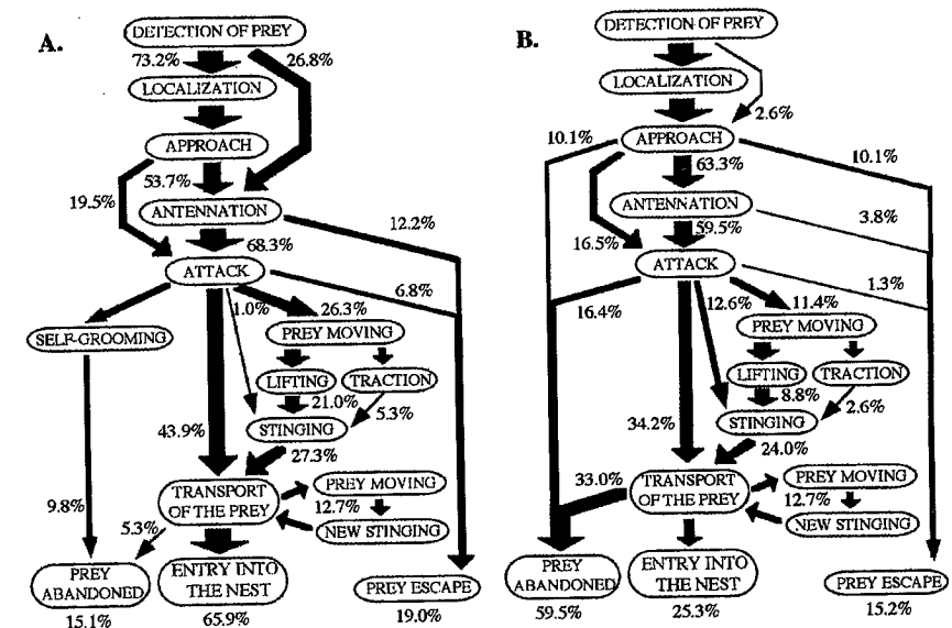
Fig. 1. Flow diagram of the A. traegordhi hunting workers when confronted with termite workers from the same log (A) (n = 205) or from a different nest site (B) (n = 79).
