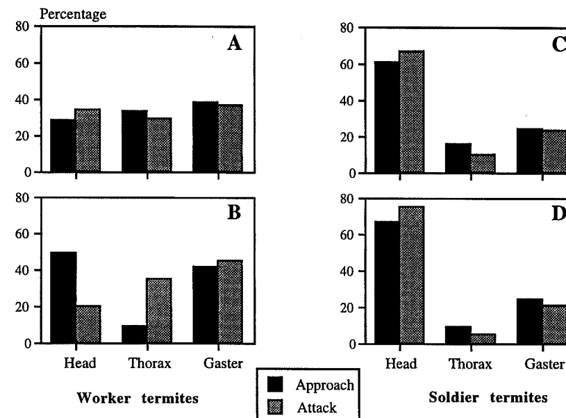
Fig. 3. Part of prey body used as a target during approach and seizure phases with termite workers living in the same log as their predator ants ( n = 180 ) (A) and from a different nest site ( n = 60 ) (B), and with termite soldiers from the same log ( n = 166 ) (C) and from a different nest site ( n = 130 ) (D).
