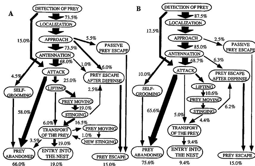
Fig. 2. Flow diagram of the A. traerghordi hunting workers when confronted with termite soldiers from the same log (A) ( n = 200 ) or from a different nest site (B) ( n = 160 ).
