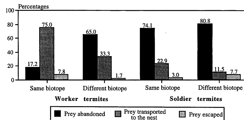
Fig. 4. Proportions of prey abandoned, transported to the nest or escaped from all prey attacked in the cases of the four prey types.
