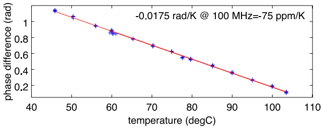
FIG. 4. Experimental phase difference versus temperature plot.
