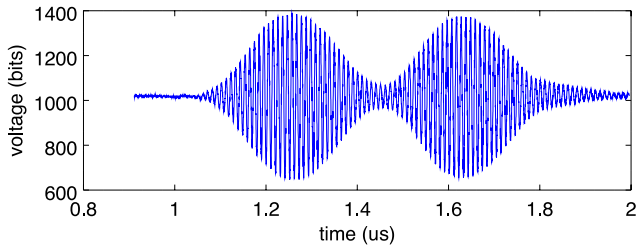
FIG. 3. Time-domain plot of the echoes returned by the acoustic wave transducer. Notice that the chart only starts after 900 ns — as do the data acquisitions — since sensor design yields no signal prior to this time offset.
