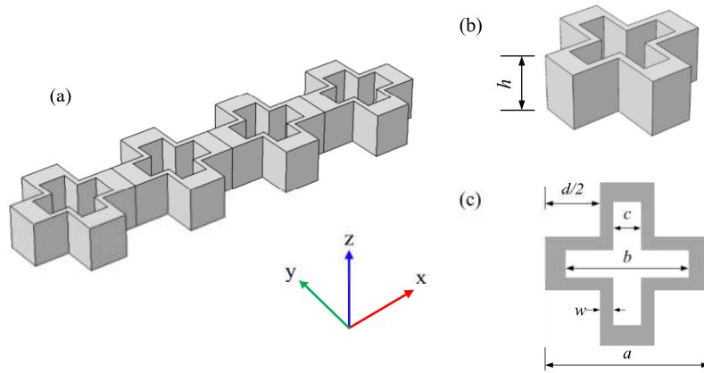
Figure 1. (a) Schematic of the cross-like holey PnC strip with the orientation of (100) -oriented silicon wafer. (b) Primitive unit cell. (c) Plane view of the unit cell with definition of geometry parameters.
