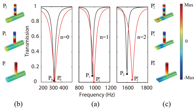
FIG. 2. Case of a single resonator. (a) Numerical transmission is plotted around the 0th, 1st, and 2nd acoustic resonances of a single resonator grafted onto the waveguide. The black and red lines are for no water ( h_w = 0 ) and half-water ( h_w = d/2 ), respectively. (b-c) Vibration modes at resonant frequencies are shown. The color scale represents the amplitude of the pressure normalized to the maximum (Max).
