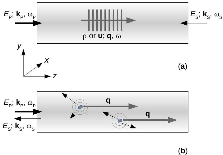
Figure 1. Brillouin light scattering (BLS) in an optical fiber or an optical waveguide, in the counter-propagating interaction setting. (a) The coherent mixing of two optical waves produces a dynamical acoustic wave grating satisfying the phase-matching conditions \omega = \omega_p - \omega_s and q = k_p - k_s . The signal wave can experience a gain from BLS of the pump wave on the dynamic grating. (b) Spontaneous Brillouin scattering occurs for photons of an incident optical wave on thermally generated acoustic phonons. The random phonons are modeled as arising from a stochastic body force distributed in the whole solid. Some of them pick up the phase-matched wavevector q .
