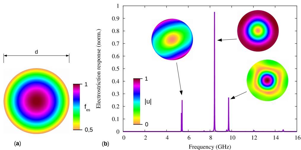
Figure 3. Electrostriction response of a silica microwire. (a) The cross-section of the microwire is circular and the diameter is d = 800 nm. The incident optical field is a Gaussian wave (normalized square modulus is shown). (b) The electrostriction response, computed as the total energy of the solution of the elastodynamic equation, is shown as a function of frequency. Examples of the solution field (norm of the total displacement) are shown for the three main peaks in the response.
