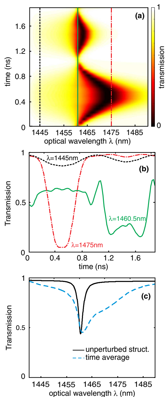
Fig. 5. AO modulation under full flexural motion. The modulation of the optical transmission spectrum is evaluated for the fundamental acoustic mode. The instantaneous optical spectrum is shown in (a) as a function of time (see Visualization 1). Three cross sections at constant optical wavelength are shown in (b) following the dotted lines in (a) (see Visualization 2). The time-averaged transmission spectrum is compared in (c) to transmission without deformation.
