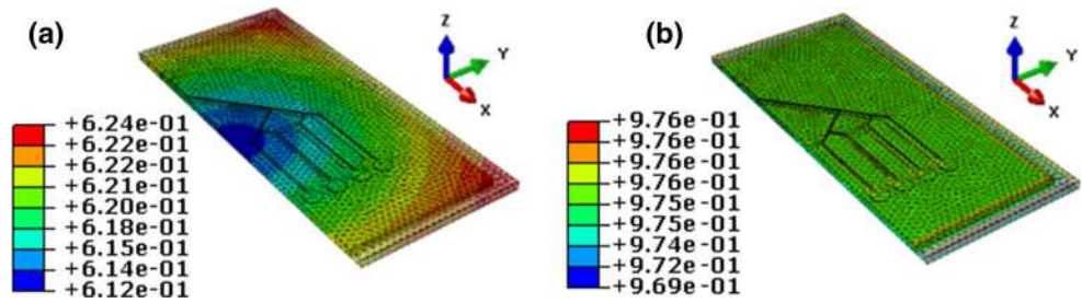
Fig. 14 Final distribution of the relative density in micro-fluidic specimens of 316L stainless steel powders, obtained after a injection molding process and b sintering stage at 1360 °C (solid loading: 60%, heating rate: 15 °C/min, hold time: 120 min)
