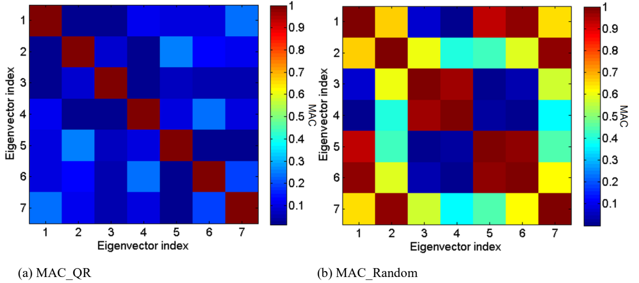
Fig. 4: MAC matrices of the QR reduced model (MAC_QR) and the randomly reduced model (MAC_Random)
