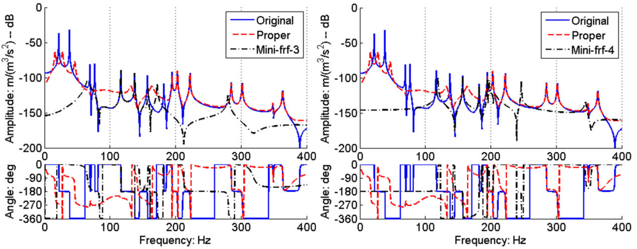
(c) Mini-frf-3 calibrated in sub-range 100-150 Hz;
