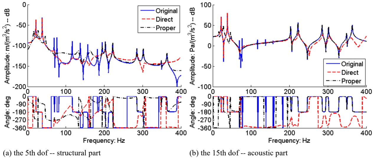
Fig. 6: The original, direct, and proper FRFs of the 5 th and 15 th dofs for Config-2
