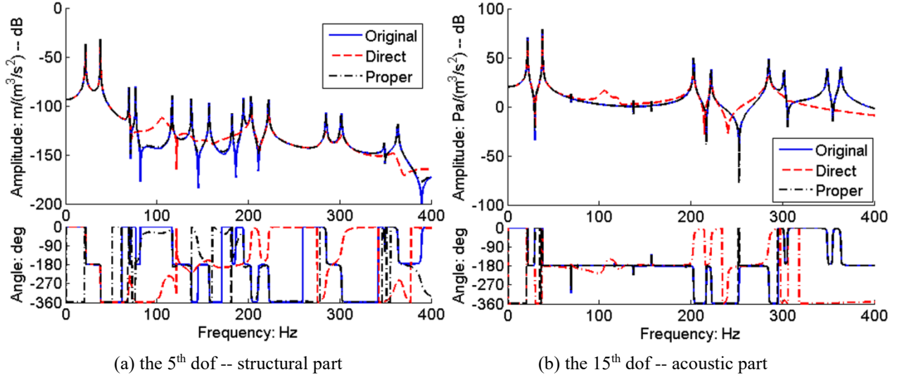
Fig. 5: The original, direct, and proper FRFs of the 5 th and 15 th dofs for Config-1
