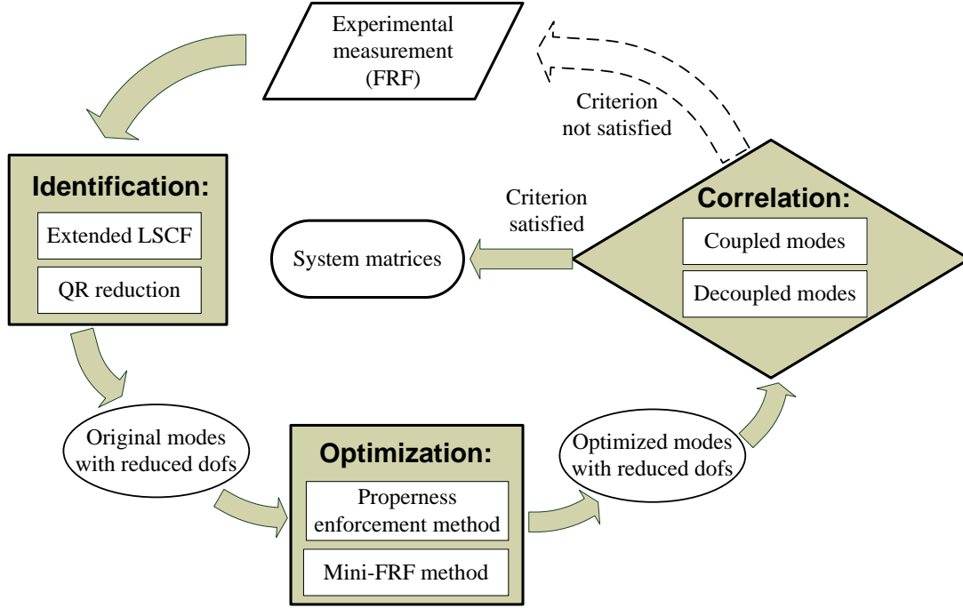
Fig. 1: The integrated framework for vibroacoustical identification
