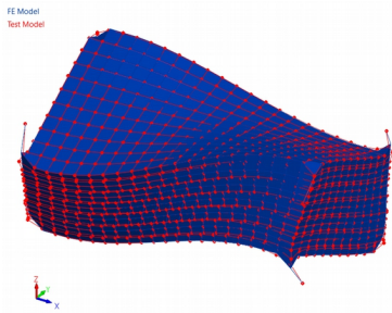
mode pair 1 – 3,073 Hz
