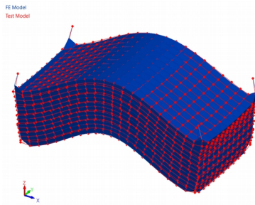
mode pair 2 – 3,428 Hz
