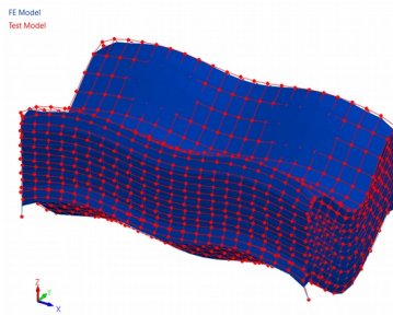
mode pair 8 – 7,681 Hz
