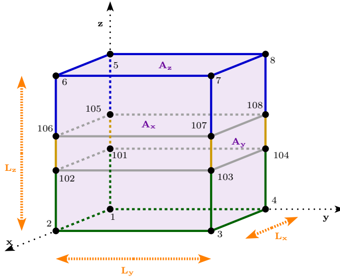
Figure 1: Structure geometry
