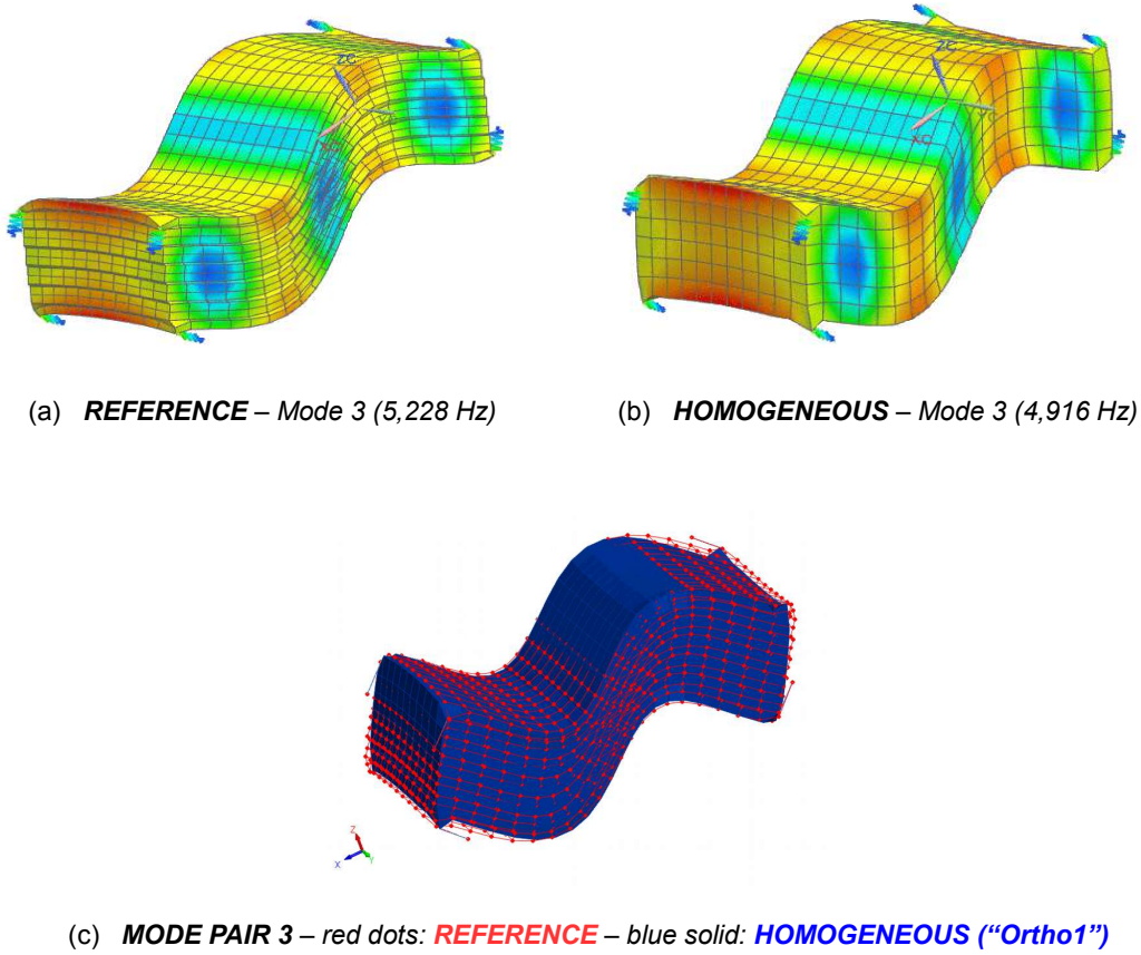
Figure 6: Compared models’ deformed shapes ((a): reference, (b): homogeneous, (c): mode pair)
