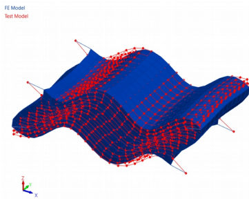
mode pair 7 – 7,329 Hz
