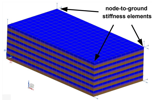
Figure 5: Global laminated reference structure
