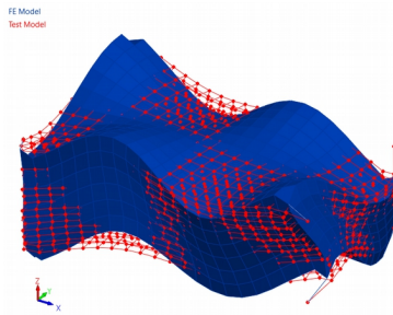
mode pair 5 – 6,809 Hz
