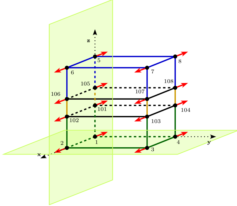
Figure 2: Pure tension along x
