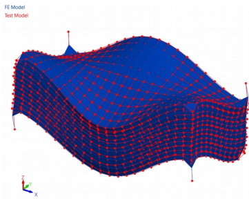
mode pair 4 – 5,374 Hz
