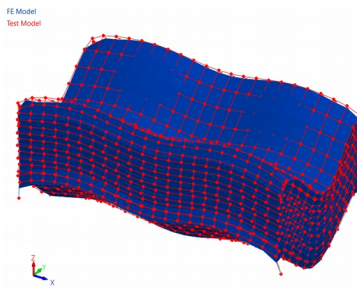
mode pair 8 – 7,681 Hz
