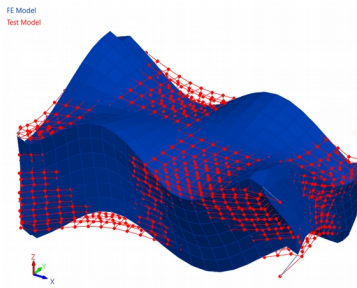
mode pair 5 – 6,809 Hz
