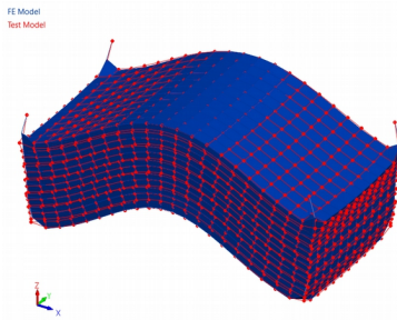
mode pair 2 – 3,428 Hz
