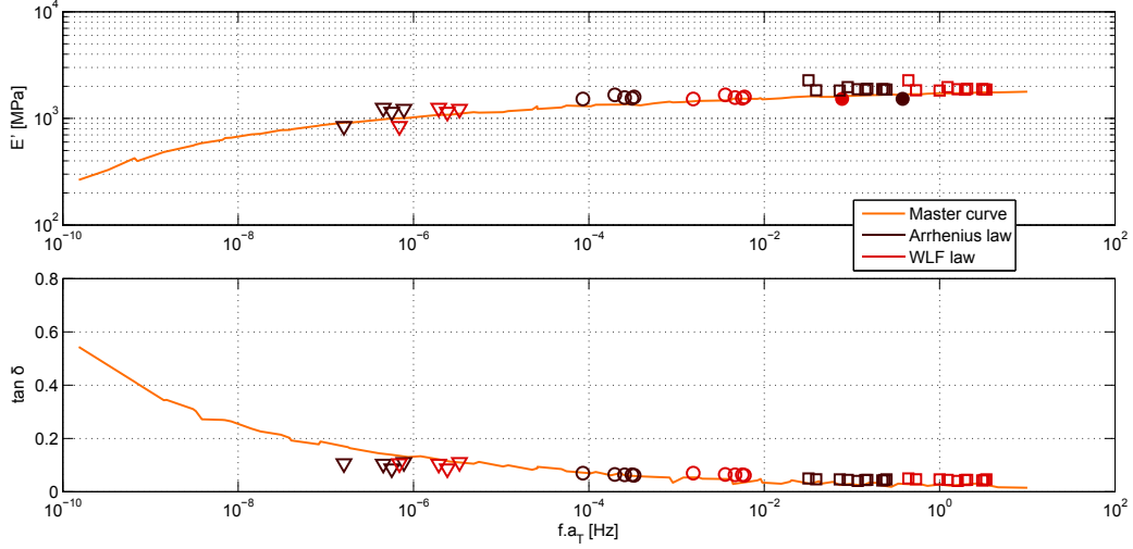
Figure 14: Comparison of the three experimental methods on the storage modulus and the loss factor according to the reduced frequency and for the reference temperature T_0 = 26^\circ \text{C} : experimental data from quasi-static tensile test at 21^\circ \text{C} (●), modal analysis at 40^\circ \text{C} (□), at 50^\circ \text{C} (○) and at 60^\circ \text{C} (▽).
