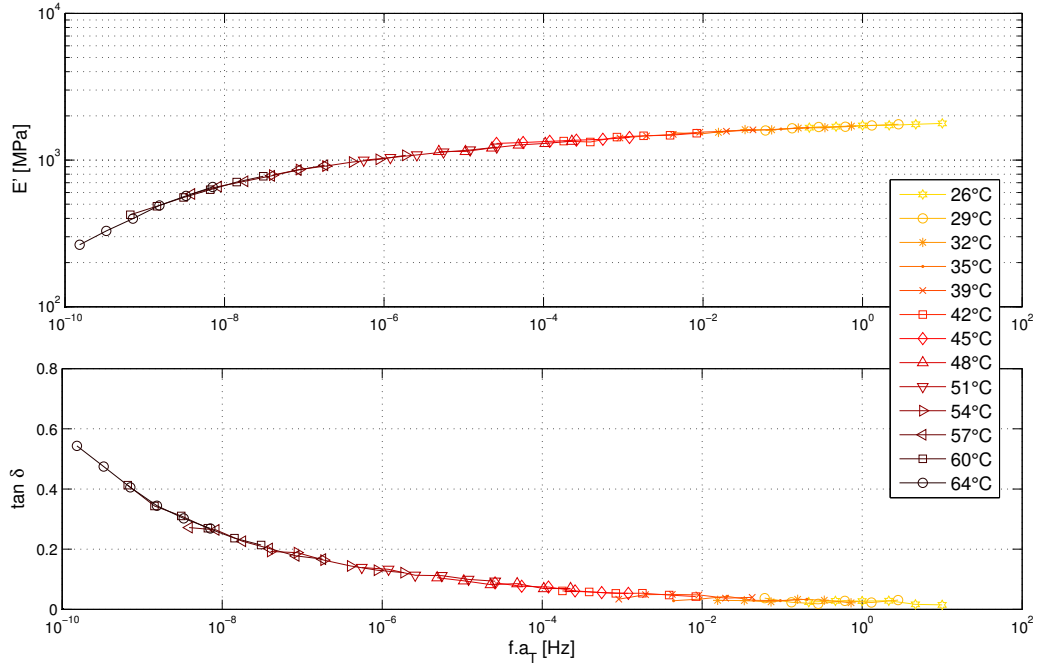
Figure 8: Master curves of E' and \tan(\delta) versus the reduced frequency f \cdot a_T with a reference temperature of 26 ° C.
