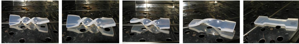
Figure 2: Shape memory demonstration of the Veriflex®, the specimen autonomously returns to its original permanent shape when heated at 120 °C.
