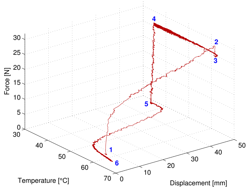
Figure 1: Cyclic thermo-mechanical test of the Veriflex®, (1-3) deformation at high temperature, (3-4) fixing temporary shape, (4-5) unloading, (5-6) shape recovery, difference between 1 and 6 is the residual deformation.
