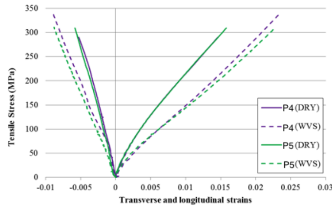
Figure 3. Tensile stress-strain curves for 0°UD specimens before and after aging
