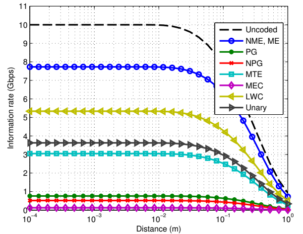
Fig. 3. Information rate for various codes, in theory.
