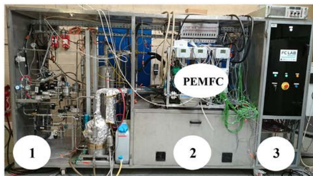
Fig. 1 – 10 kW test bench.
