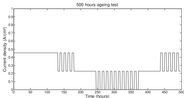
Fig. 8 – 500 h \mu -CHP load profile.
