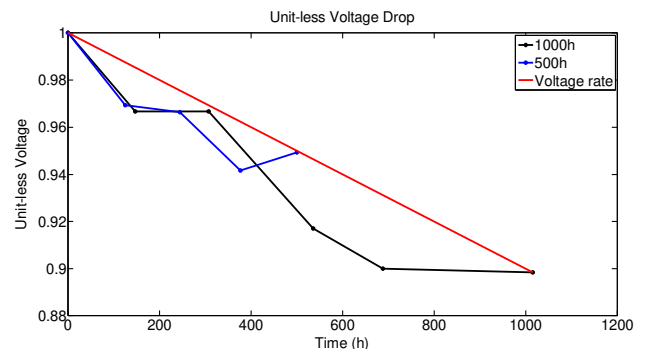
Fig. 12 – Unit-less voltage drop and degradations rate comparison for 1,000 h and 500 h tests.
