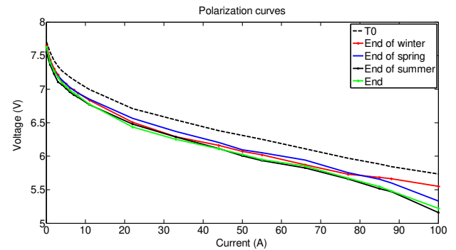
Fig. 10 – Ageing impact on the polarization curves obtained during the reduced test (500 h).
