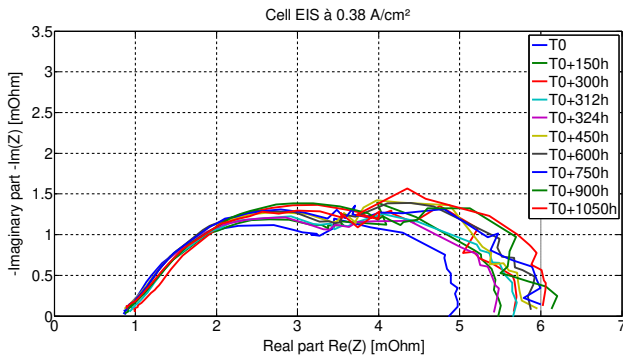
Fig. 7 – Ageing impact on the EIS measurements (1000 h).
