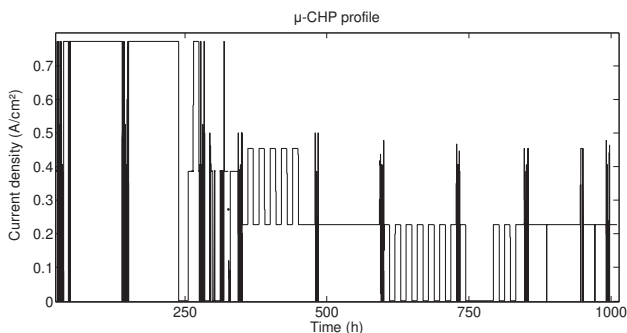
Fig. 4 – 1000 h \mu -CHP load profile.
