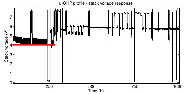
Fig. 5 – Stack voltage response (1000 h test).
