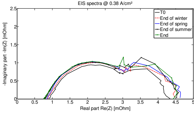
Fig. 11 – Ageing impact on the EIS measurements.
