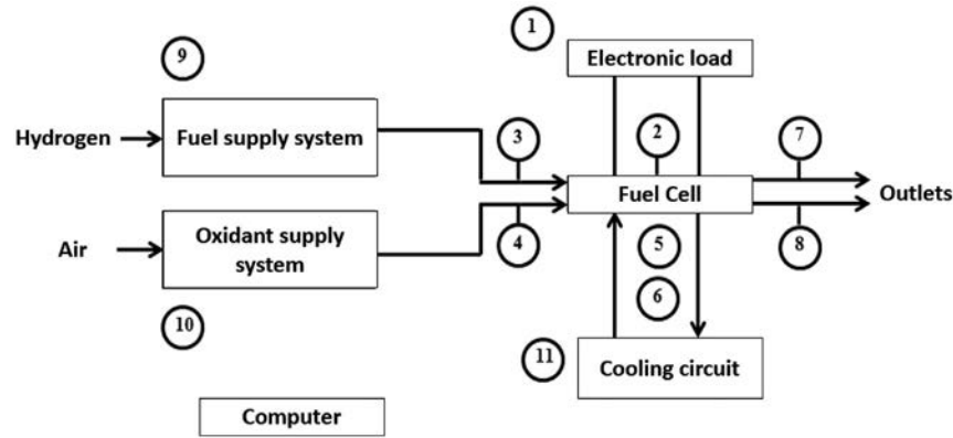
Fig. 2 – Locations of the different sensors on the test bench.
