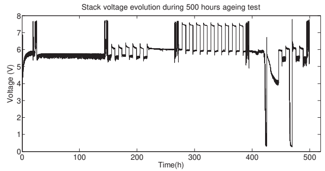
Fig. 9 – Stack voltage response (500 h test).
