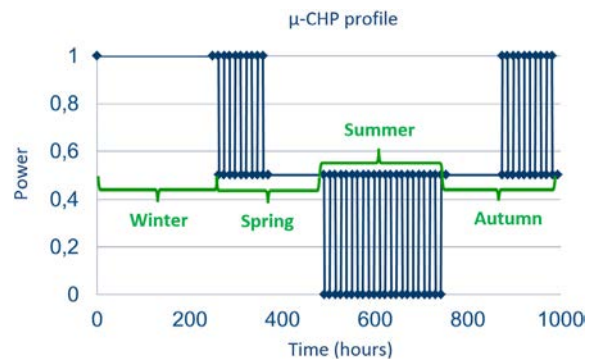
Fig. 3 – \mu -CHP normalized power profile.
