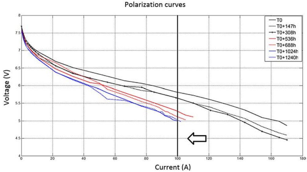
Fig. 6 – Ageing impact on the polarization curves (1000 h test).
