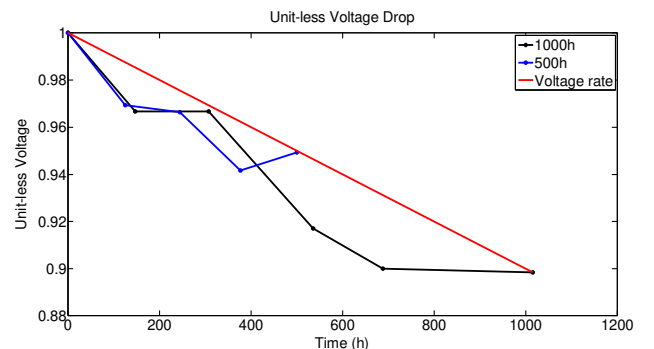
Fig. 12 – Unit-less voltage drop and degradations rate comparison for 1,000 h and 500 h tests.
