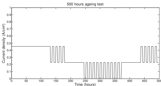
Fig. 8 – 500 h \mu -CHP load profile.
