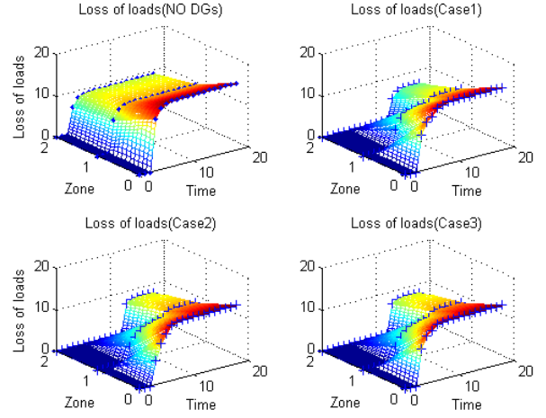
Fig. 4. Loss of load vs. zone and time.
