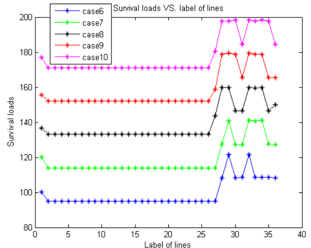
Fig. 7. Surviving loads vs. label of hardening line cases.
