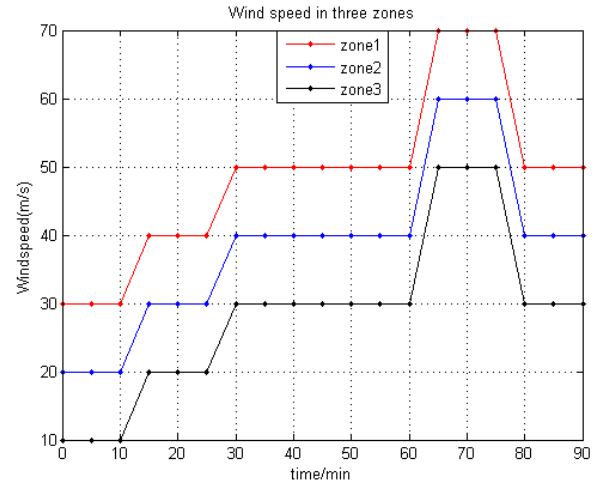
Fig. 3. Wind speed profiles.
