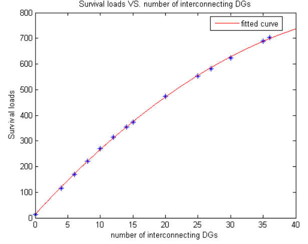
Fig. 6. Surviving loads vs. number of connected DG sources.
