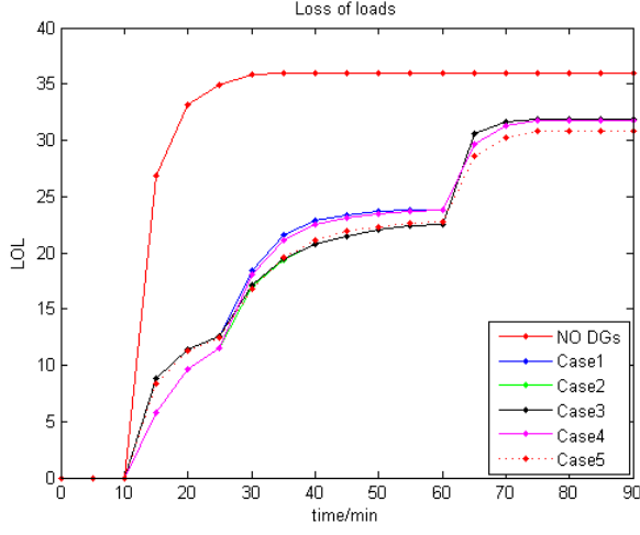
Fig. 5. Average loss of load vs. time
