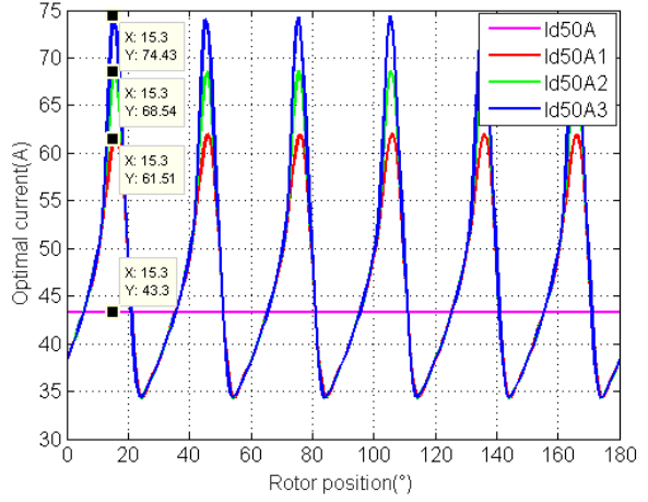
Fig. 18 Optimal currents I_a
