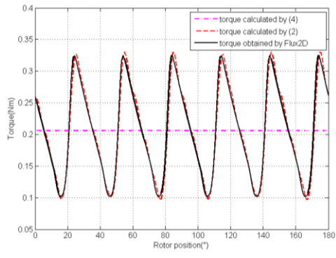
Fig. 3 Torques obtained by Flux 2D and calculations
