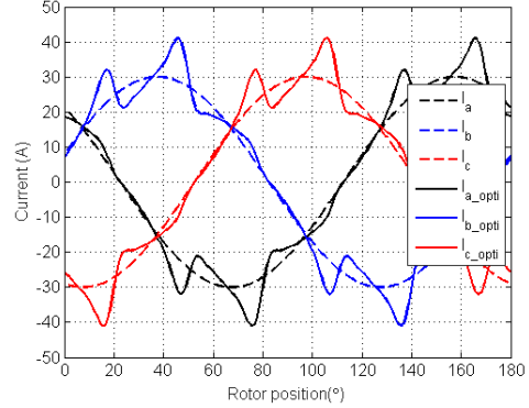
Fig. 7 The optimal currents of stator
