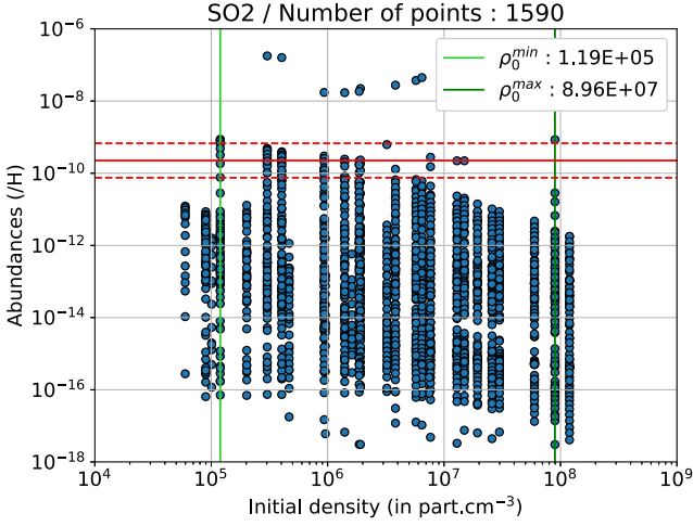
Figure 8. Comprehensive example of the application of the method on observed \text{SO}_2 in IRAS 16293–2422. The horizontal red line represents the observed abundance relative to H of 2.25 \times 10^{-10} and the dashed ones its uncertainty factor of 3. The light and dark green vertical lines respectively represent the minimal and maximal values of the initial density \rho_0 that are constrained by the observed abundance.
