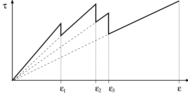
Fig. 2. A strain-controlled experiment. The solid line is the load path followed during the experiment. The dashed lines represent the path that would be followed if strain were to be decreased at some point during the experiment. When a fiber breaks at constant \varepsilon , the load \tau must be reduced as represented by the vertical drops.
