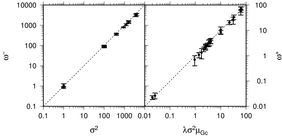
Figure 8. Comparisons between the predicted values of the energy release rate power spectrum P_G(k) and the observed values in the simulations. Predictions of the values of P_G(k) are given at large scale by Eq. (6.40) and are compared to values extracted from simulations results \omega^+ . At small scale analytical results predicted by Eq. (6.20) are compared to the values \omega^- corresponding to the plateau P_G(k) in simulations.
