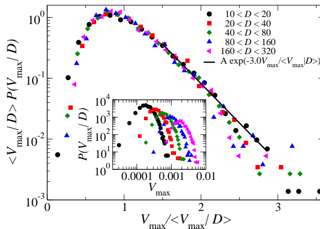
Figure 9. The inset shows the distributions P(V_{\max} | D) at various fixed durations D -ranges. The main panel demonstrates that these distribution can be collapsed, when plotting \langle V_{\max} | D \rangle P(V_{\max} | D) as a function of V_{\max} / \langle V_{\max} | D \rangle in a semi-log scale. The scaling function has a clear exponential tail different from the power-law behavior of the experimental data.
