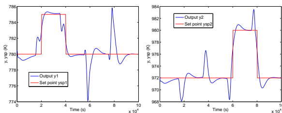
Figure 9: DMC control with H_{p,low} = 10 . Left: Riser temperature (K). Right: Regenerator temperature (K).
