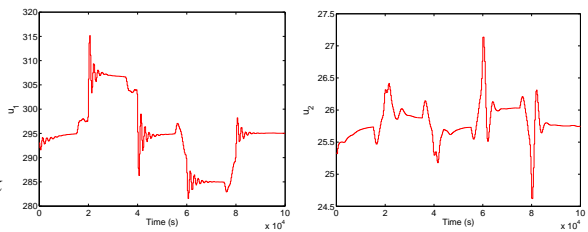
Figure 8: DMC control with H_{p,low} = 1 . Left: Catalyst flow rate (kg/s). Right: Air flow rate (kg/s).
