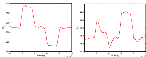
Figure 18: Observer Based Model Predictive Control with H_p = 20 , H_{p,low} = 1 , \sigma_y = 0.5 . Left: Catalyst flow rate (kg/s). Right: Air flow rate (kg/s).
