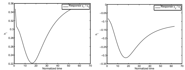
Figure 5: Unit step response coefficients for both outputs with respect to manipulated mass flow rate of catalyst
