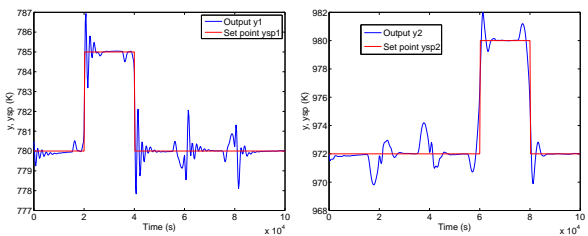
Figure 7: DMC control with H_{p,low} = 1 . Left: Riser temperature (K). Right: Regenerator temperature (K).
