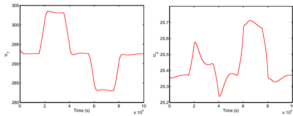
Figure 16: Observer Based Model Predictive Control with H_p = 20 , H_{p,low} = 1 , \sigma_y = 0.01 . Left: Catalyst flow rate (kg/s). Right: Air flow rate (kg/s).
