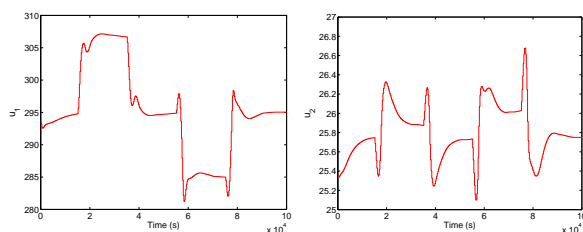
Figure 10: DMC control with H_{p,low} = 10 . Left: Catalyst flow rate (kg/s). Right: Air flow rate (kg/s).
