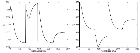
Figure 4: Responses of top riser temperature and regenerator temperature used for open loop identification
