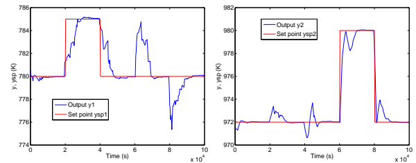
Figure 13: Nonlinear MPC control with H_p = 3 , H_c = 1 . Left: Riser temperature (K). Right: Regenerator temperature (K).
