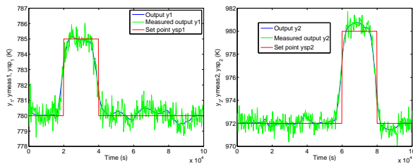
Figure 17: Observer Based Model Predictive Control with H_p = 20 , H_{p,low} = 1 , \sigma_y = 0.5 . Left: Riser temperature (K). Right: Regenerator temperature (K).
