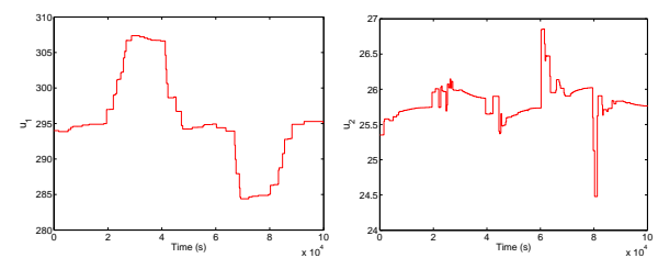
Figure 14: Nonlinear MPC control with H_p = 3 , H_c = 1 . Left: Catalyst flow rate (kg/s). Right: Air flow rate (kg/s).
