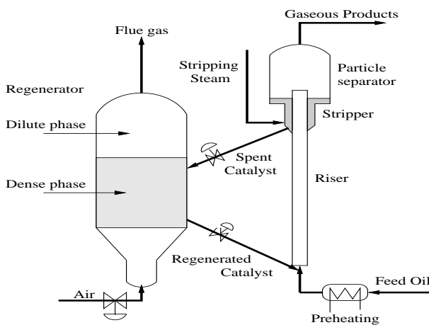
Figure 1: Schematic diagram of a FCC unit
