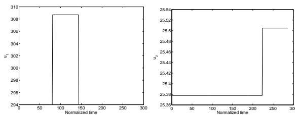
Figure 3: Mass flow rate of catalyst and mass flow rate of air imposed for open loop identification
