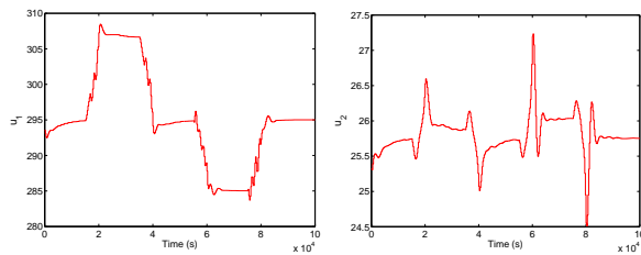
Figure 12: MPC control with nonlinear optimization by NLPQL and H_{p,low} = 1 . Left: Catalyst flow rate (kg/s). Right: Air flow rate (kg/s).
