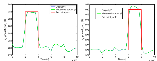
Figure 15: Observer Based Model Predictive Control with H_p = 20 , H_{p,low} = 1 , \sigma_y = 0.01 . Left: Riser temperature (K). Right: Regenerator temperature (K).
