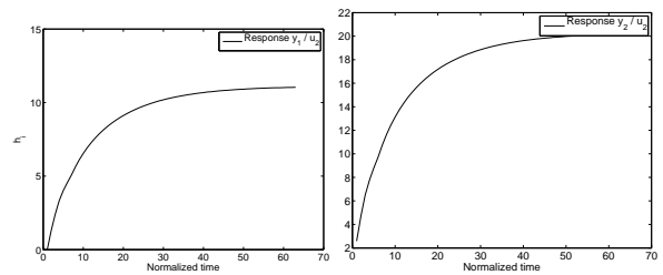
Figure 6: Unit step response coefficients for both outputs with respect to manipulated mass flow rate of air
