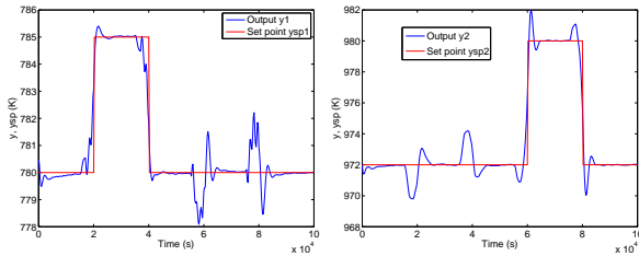
Figure 11: MPC control with nonlinear optimization by NLPQL and H_{p,low} = 1 . Left: Riser temperature (K). Right: Regenerator temperature (K).
