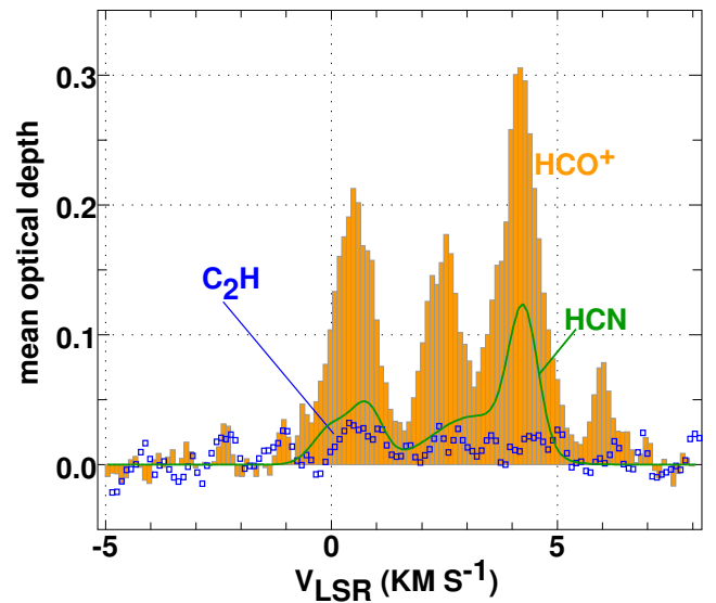
Fig. 5. Mean optical depth profiles for strongly polar molecules for the eight sources with N(DNM) \geq 2 \times 10^{20} \text{ cm}^{-2} . The HCN profile in green shows the kinematic structure that would be convolved with the HCN hyperfine splitting to reproduce the observations assuming that the hyperfine components appear in the LTE ratio 5:3:1. C 2 H is shown in blue.
