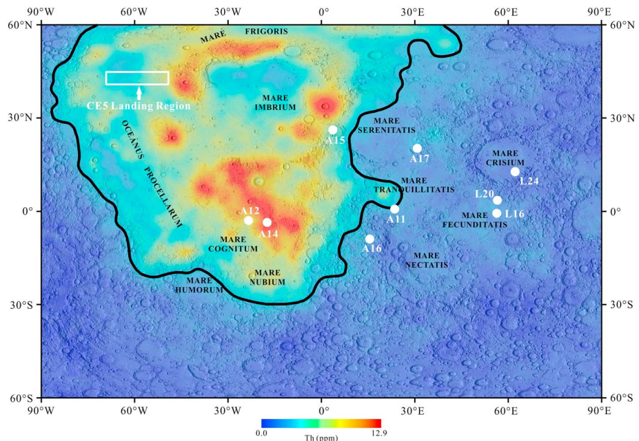
Figure 2. Thorium abundance map of the lunar nearside. The thick black line denotes the boundary of the Procellarum KREEP Terrane ( Th > 3.5 ppm). “A” represents the Apollo sampling sites; “L” represents the Luna sampling sites. The white box indicates the CE5 designated landing region. The basemap is a Lunar Orbiter Laser Altimeter and Kaguya Terrain Camera merged hillshade map (Barker et al., 2016) superposed on the Lunar Prospector thorium data (Prettyman et al., 2006).
