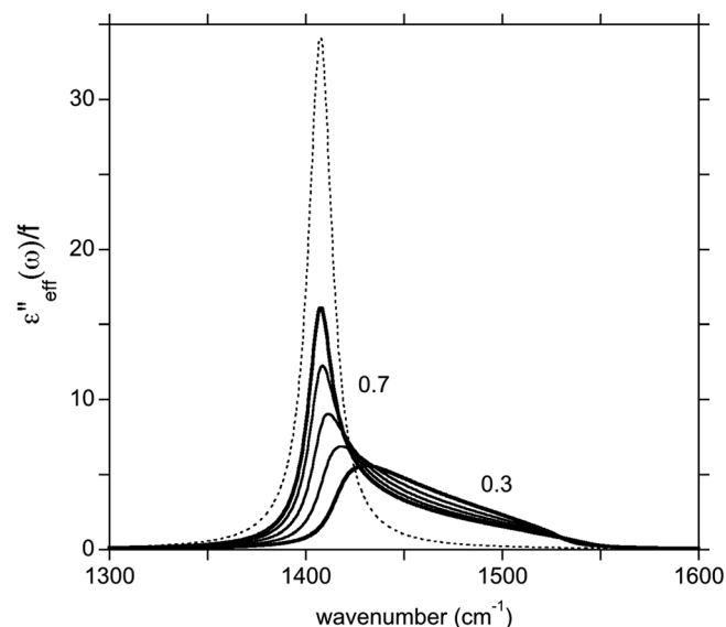
Fig. 4. Imaginary part of effective dielectric function in the \nu_3\text{CO}_3 range computed using the classical expression of the calcite dielectric tensor and the Bruggeman model for a volume fraction of calcite varying from 0.3 to 0.7 by steps of 0.1. The effective dielectric functions have been divided by the corresponding volume fraction. The imaginary part of the dielectric function of pure calcite corresponding to the \nu_3\text{CO}_3 mode is reported for comparison (dotted line).
